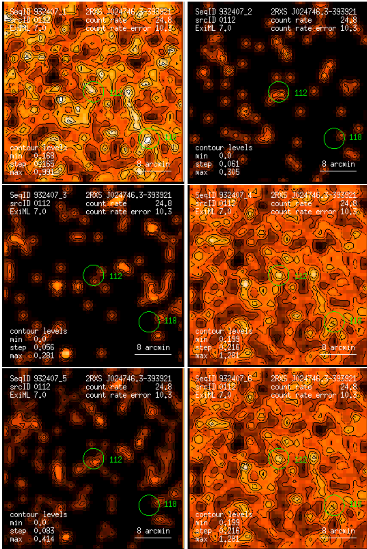
Figure 112: RASS 932407: detection 0112: band rate images, Gaussian filter: (1) PSPC channels 11 – 41, (2) 52 – 90, (3) 91 – 201, (4) 11 – 235, (5) 52 – 201, (6) 11 – 201. Broad band rates in counts/ks. Band rate contour levels in counts/ks/arcmin 2 .
