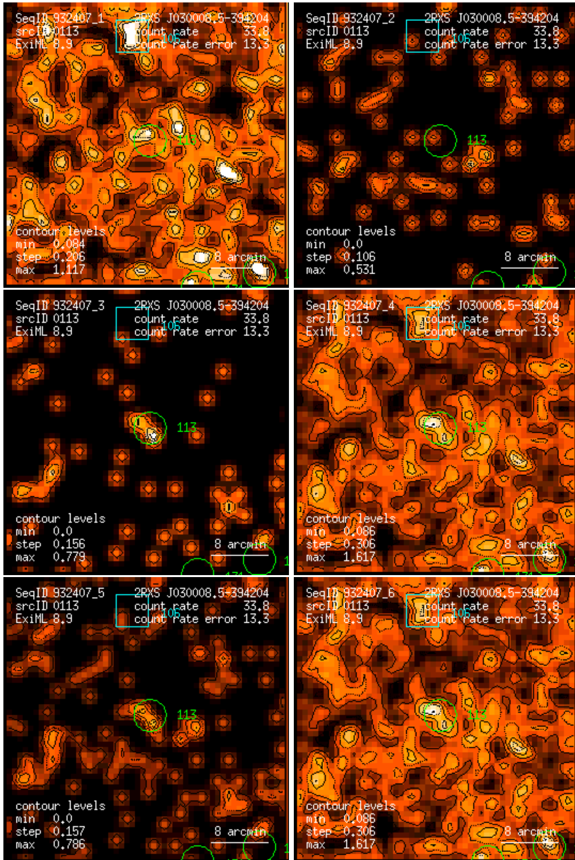
Figure 113: RASS 932407: detection 0113: band rate images, Gaussian filter: (1) PSPC channels 11 – 41, (2) 52 – 90, (3) 91 – 201, (4) 11 – 235, (5) 52 – 201, (6) 11 – 201. Broad band rates in counts/ks. Band rate contour levels in counts/ks/arcmin 2 .
