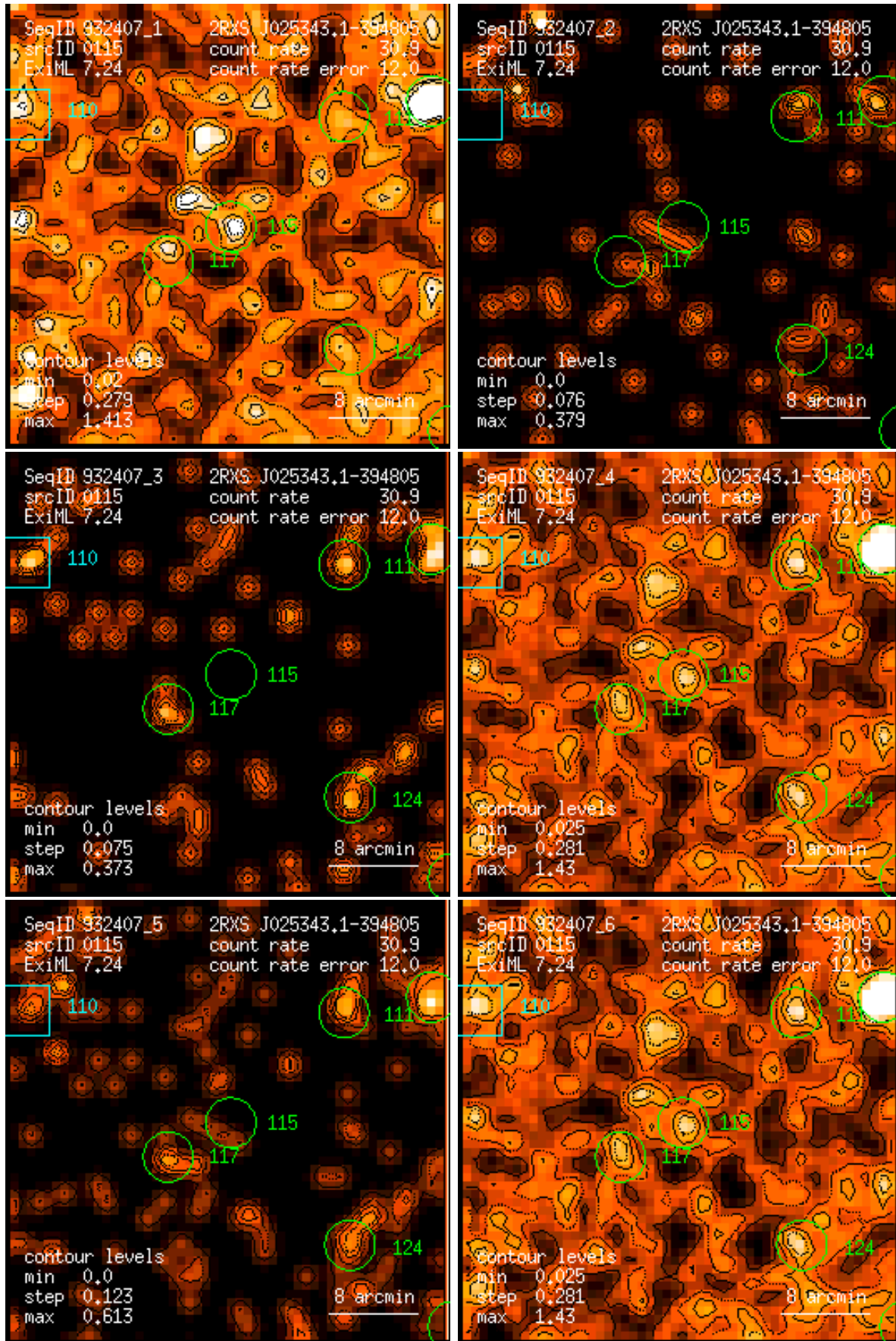
Figure 115: RASS 932407: detection 0115: band rate images, Gaussian filter: (1) PSPC channels 11 – 41, (2) 52 – 90, (3) 91 – 201, (4) 11 – 235, (5) 52 – 201, (6) 11 – 201. Broad band rates in counts/ks. Band rate contour levels in counts/ks/arcmin 2 .
