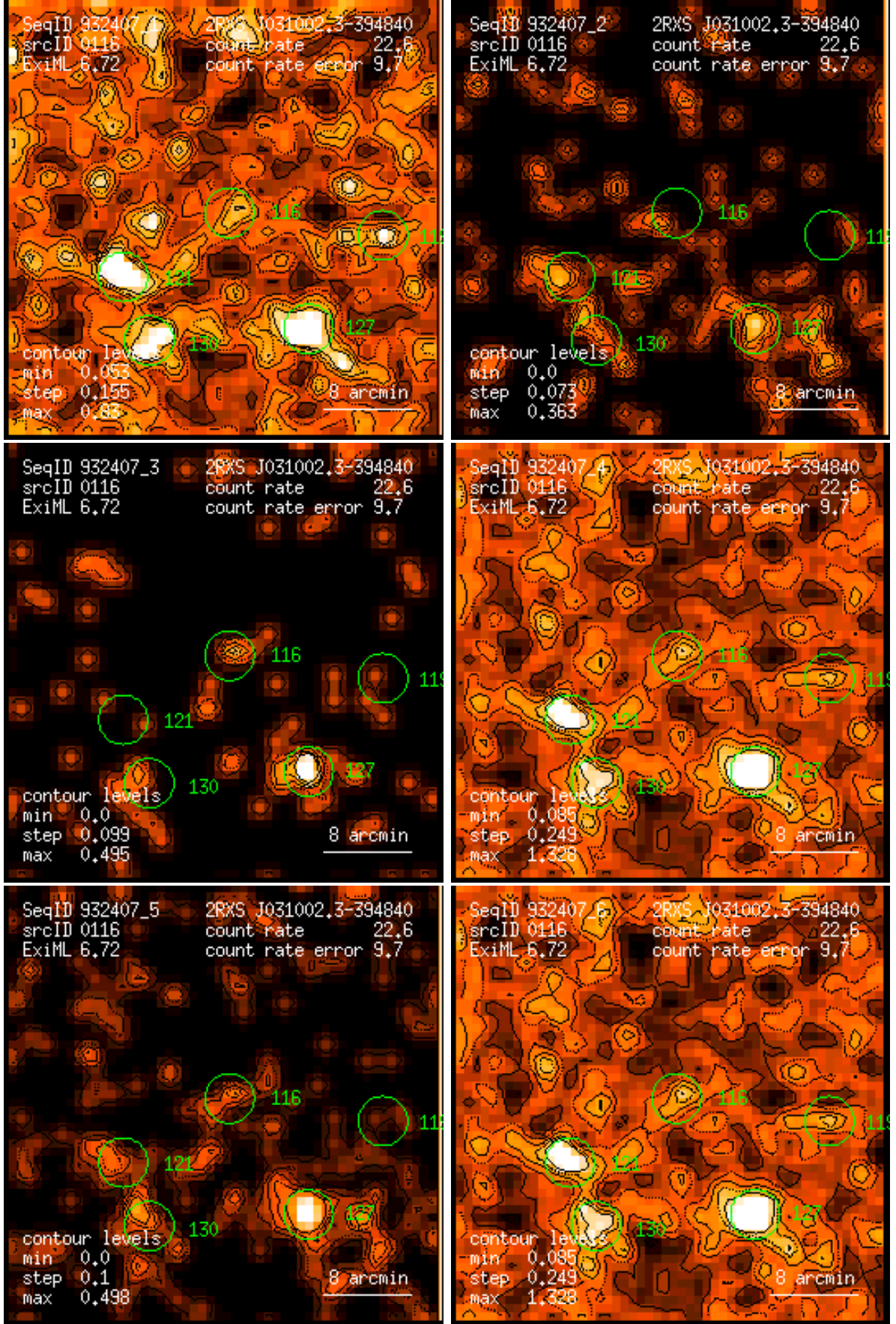
Figure 116: RASS 932407: detection 0116: band rate images, Gaussian filter: (1) PSPC channels 11 – 41, (2) 52 – 90, (3) 91 – 201, (4) 11 – 235, (5) 52 – 201, (6) 11 – 201. Broad band rates in counts/ks. Band rate contour levels in counts/ks/arcmin 2 .
