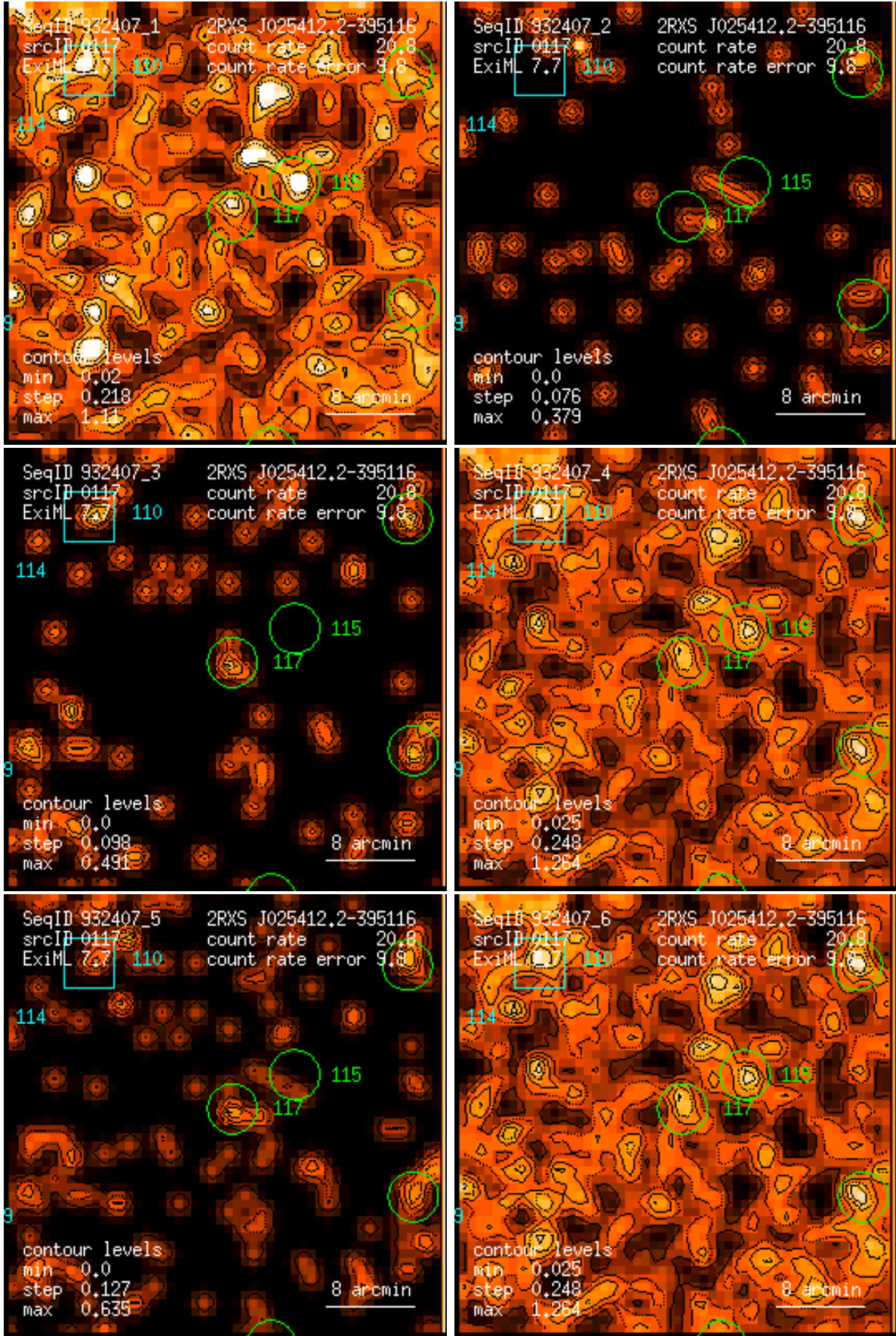
Figure 117: RASS 932407: detection 0117: band rate images, Gaussian filter: (1) PSPC channels 11 – 41, (2) 52 – 90, (3) 91 – 201, (4) 11 – 235, (5) 52 – 201, (6) 11 – 201. Broad band rates in counts/ks. Band rate contour levels in counts/ks/arcmin 2 .
