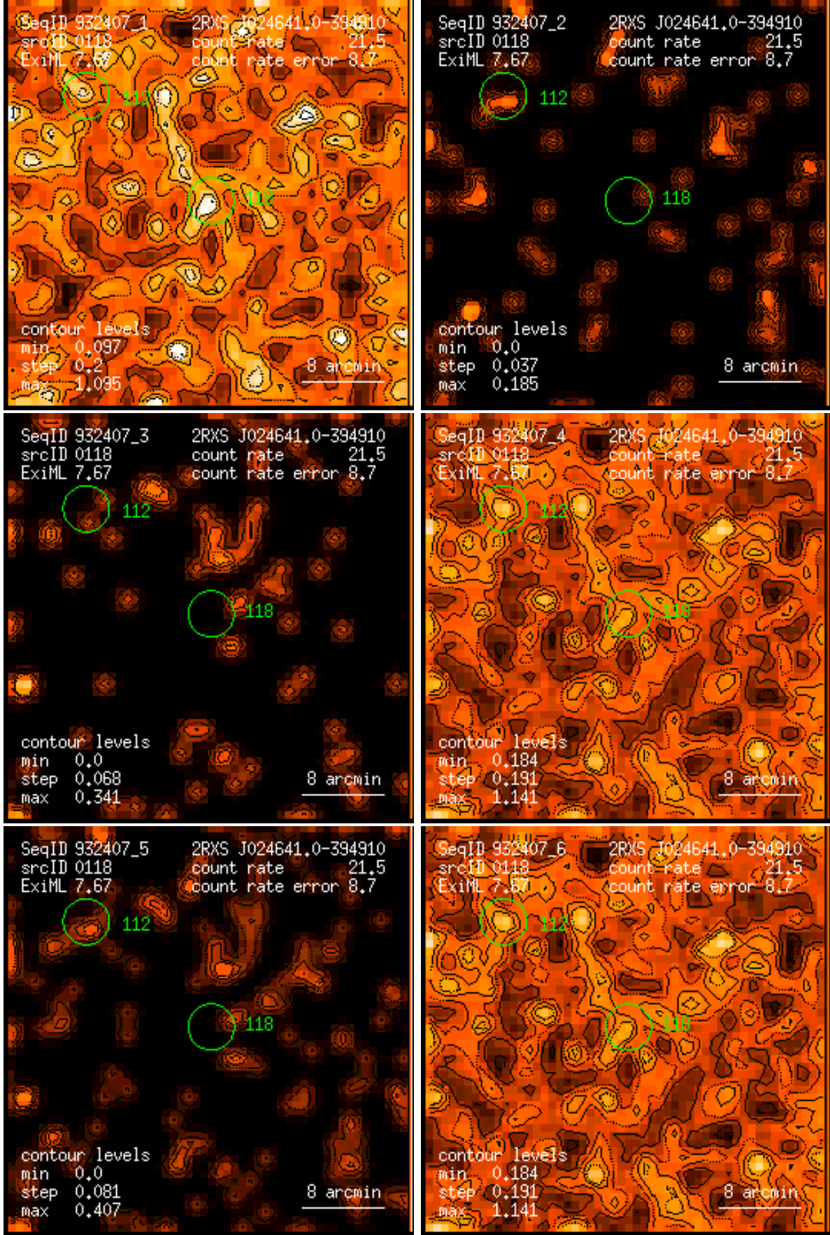
Figure 118: RASS 932407: detection 0118: band rate images, Gaussian filter: (1) PSPC channels 11 – 41, (2) 52 – 90, (3) 91 – 201, (4) 11 – 235, (5) 52 – 201, (6) 11 – 201. Broad band rates in counts/ks. Band rate contour levels in counts/ks/arcmin 2 .
