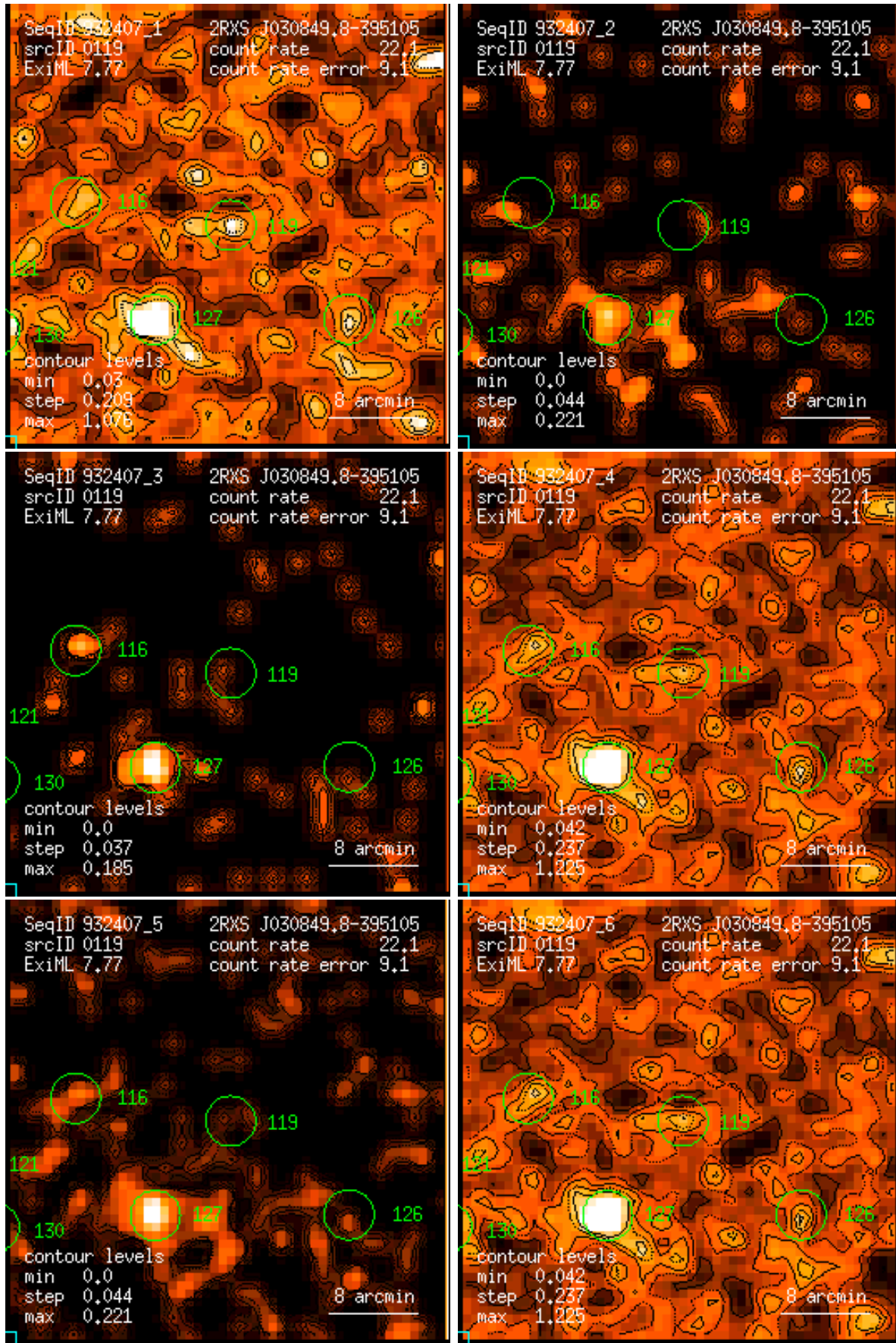
Figure 119: RASS 932407: detection 0119: band rate images, Gaussian filter: (1) PSPC channels 11 – 41, (2) 52 – 90, (3) 91 – 201, (4) 11 – 235, (5) 52 – 201, (6) 11 – 201. Broad band rates in counts/ks. Band rate contour levels in counts/ks/arcmin 2 .
