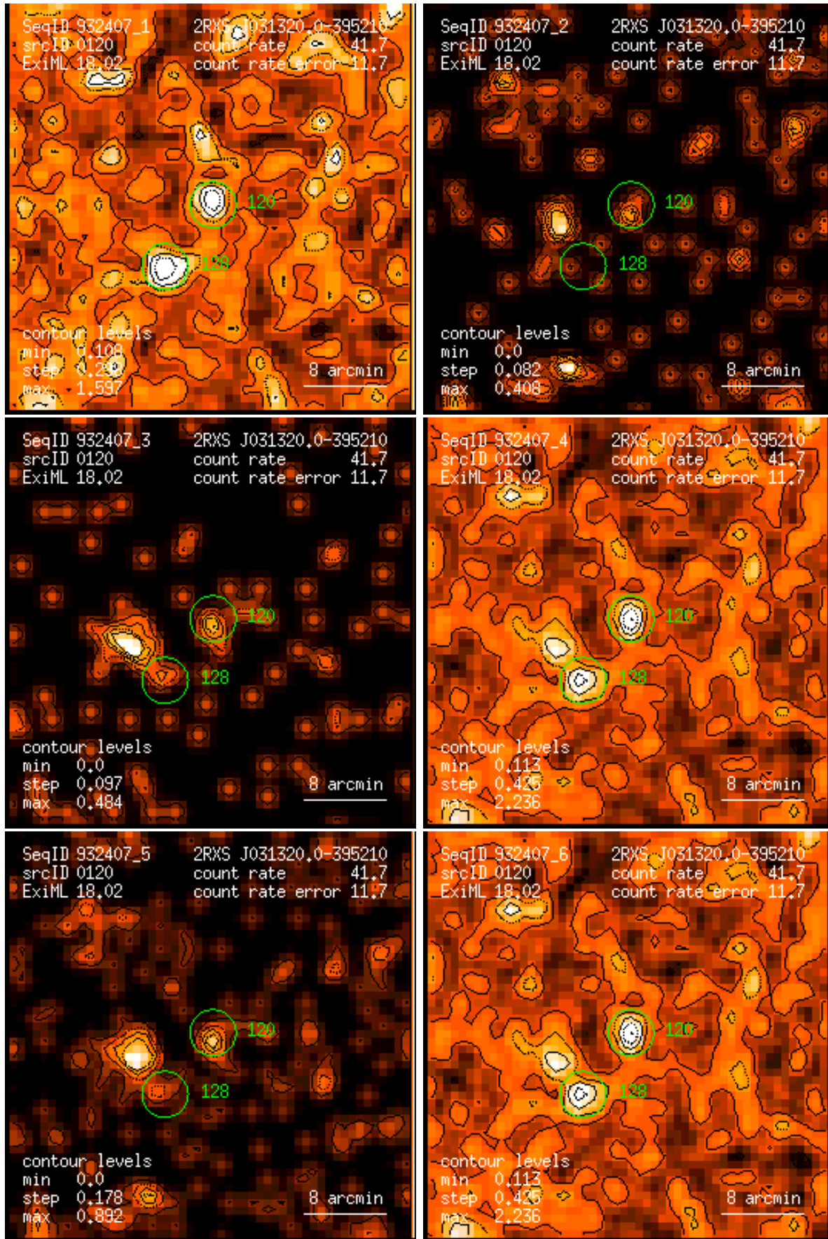
Figure 120: RASS 932407: detection 0120: band rate images, Gaussian filter: (1) PSPC channels 11 – 41, (2) 52 – 90, (3) 91 – 201, (4) 11 – 235, (5) 52 – 201, (6) 11 – 201. Broad band rates in counts/ks. Band rate contour levels in counts/ks/arcmin 2 .
