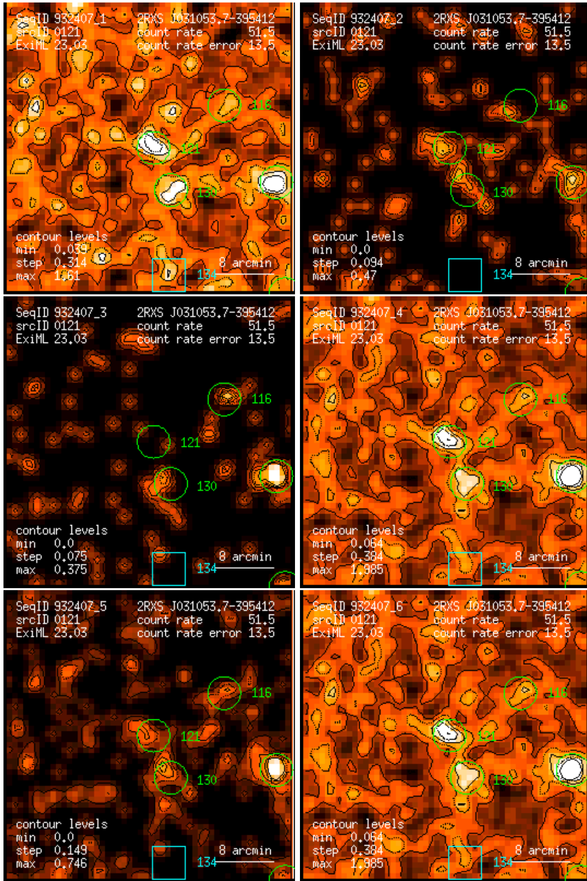
Figure 121: RASS 932407: detection 0121: band rate images, Gaussian filter: (1) PSPC channels 11 – 41, (2) 52 – 90, (3) 91 – 201, (4) 11 – 235, (5) 52 – 201, (6) 11 – 201. Broad band rates in counts/ks. Band rate contour levels in counts/ks/arcmin 2 .
