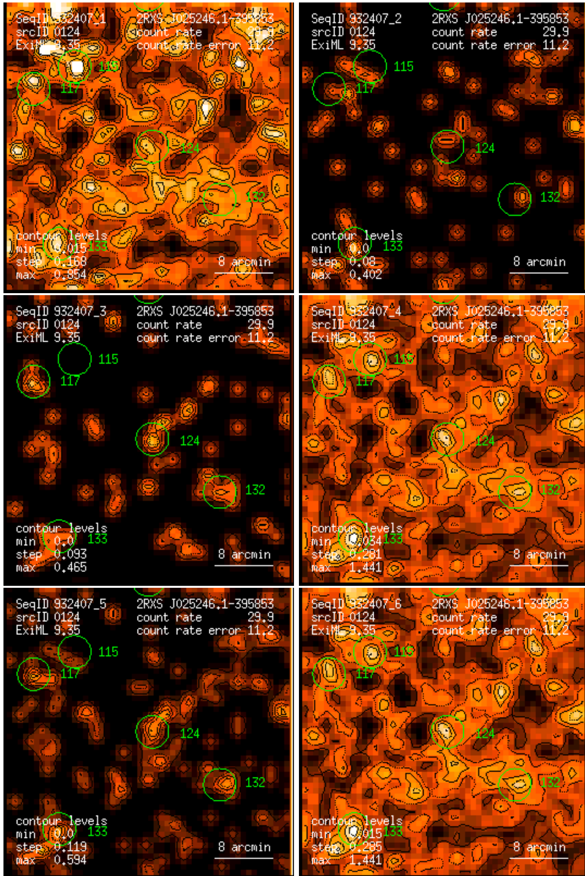
Figure 124: RASS 932407: detection 0124: band rate images, Gaussian filter: (1) PSPC channels 11 – 41, (2) 52 – 90, (3) 91 – 201, (4) 11 – 235, (5) 52 – 201, (6) 11 – 201. Broad band rates in counts/ks. Band rate contour levels in counts/ks/arcmin 2 .
