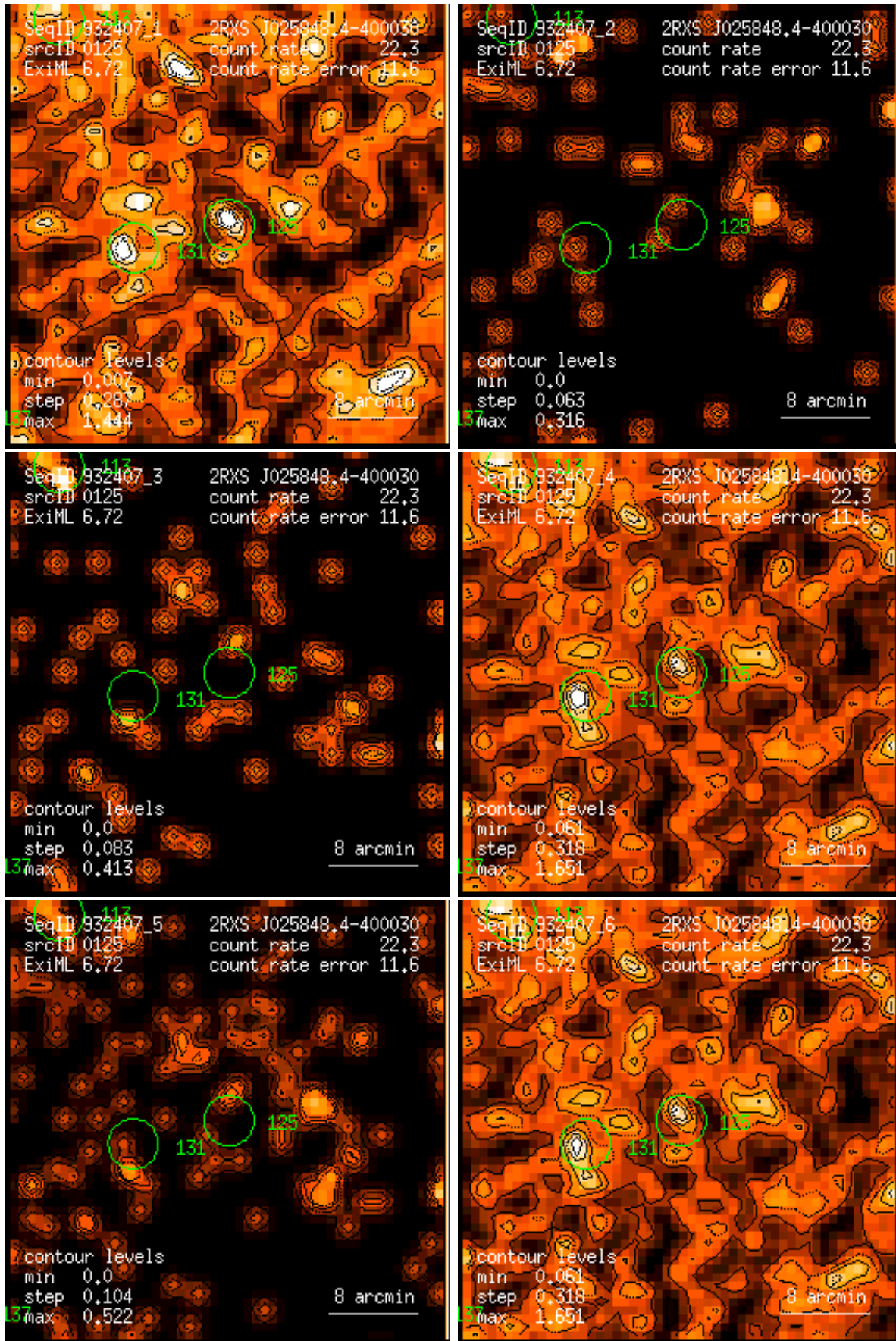
Figure 125: RASS 932407: detection 0125: band rate images, Gaussian filter: (1) PSPC channels 11 – 41, (2) 52 – 90, (3) 91 – 201, (4) 11 – 235, (5) 52 – 201, (6) 11 – 201. Broad band rates in counts/ks. Band rate contour levels in counts/ks/arcmin 2 .
