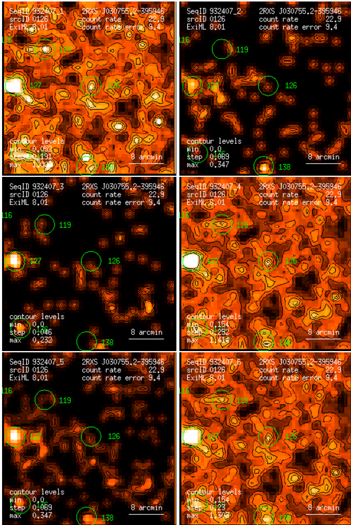
Figure 126: RASS 932407: detection 0126: band rate images, Gaussian filter: (1) PSPC channels 11 – 41, (2) 52 – 90, (3) 91 – 201, (4) 11 – 235, (5) 52 – 201, (6) 11 – 201. Broad band rates in counts/ks. Band rate contour levels in counts/ks/arcmin 2 .
