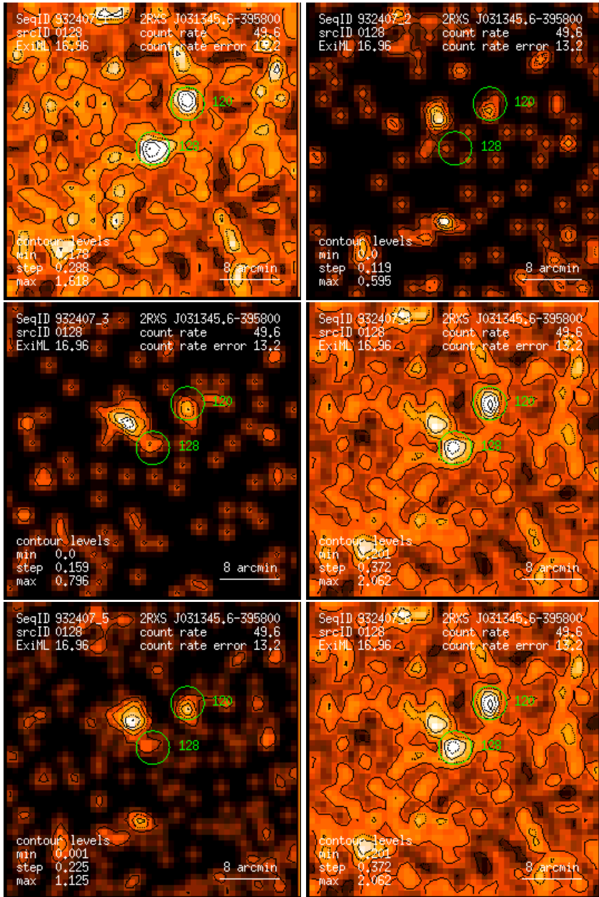
Figure 128: RASS 932407: detection 0128: band rate images, Gaussian filter: (1) PSPC channels 11 – 41, (2) 52 – 90, (3) 91 – 201, (4) 11 – 235, (5) 52 – 201, (6) 11 – 201. Broad band rates in counts/ks. Band rate contour levels in counts/ks/arcmin 2 .
