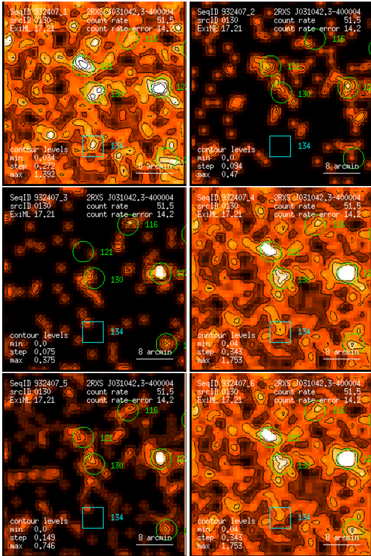
Figure 130: RASS 932407: detection 0130: band rate images, Gaussian filter: (1) PSPC channels 11 – 41, (2) 52 – 90, (3) 91 – 201, (4) 11 – 235, (5) 52 – 201, (6) 11 – 201. Broad band rates in counts/ks. Band rate contour levels in counts/ks/arcmin 2 .
