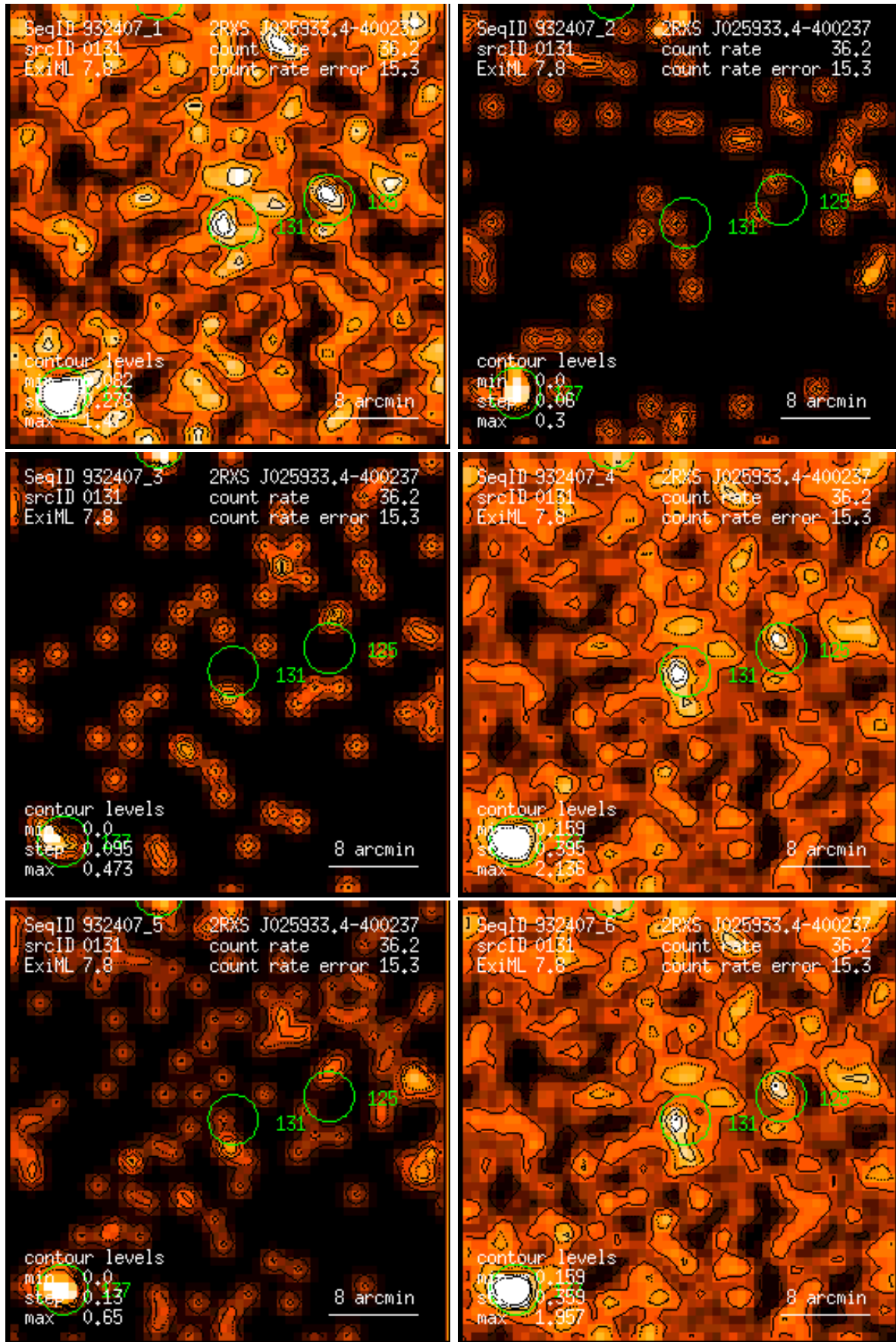
Figure 131: RASS 932407: detection 0131: band rate images, Gaussian filter: (1) PSPC channels 11 – 41, (2) 52 – 90, (3) 91 – 201, (4) 11 – 235, (5) 52 – 201, (6) 11 – 201. Broad band rates in counts/ks. Band rate contour levels in counts/ks/arcmin 2 .
