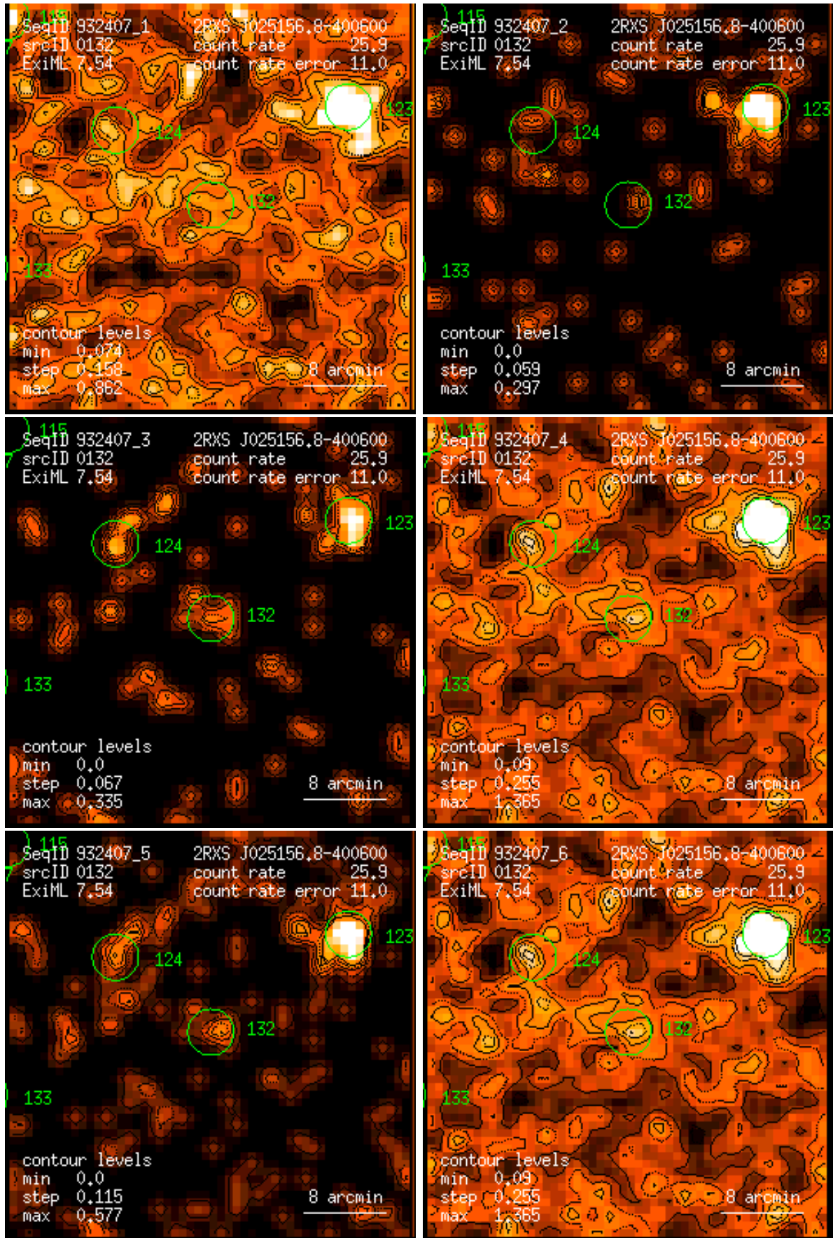
Figure 132: RASS 932407: detection 0132: band rate images, Gaussian filter: (1) PSPC channels 11 – 41, (2) 52 – 90, (3) 91 – 201, (4) 11 – 235, (5) 52 – 201, (6) 11 – 201. Broad band rates in counts/ks. Band rate contour levels in counts/ks/arcmin 2 .
