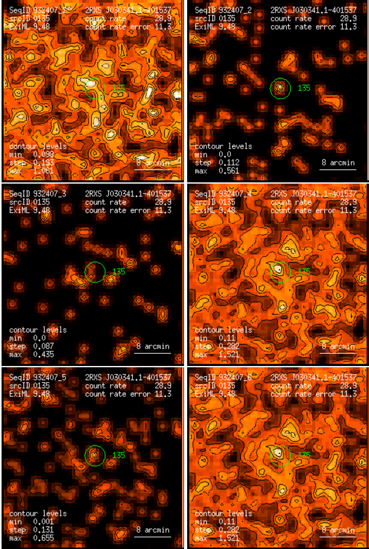
Figure 135: RASS 932407: detection 0135: band rate images, Gaussian filter: (1) PSPC channels 11 – 41, (2) 52 – 90, (3) 91 – 201, (4) 11 – 235, (5) 52 – 201, (6) 11 – 201. Broad band rates in counts/ks. Band rate contour levels in counts/ks/arcmin 2 .
