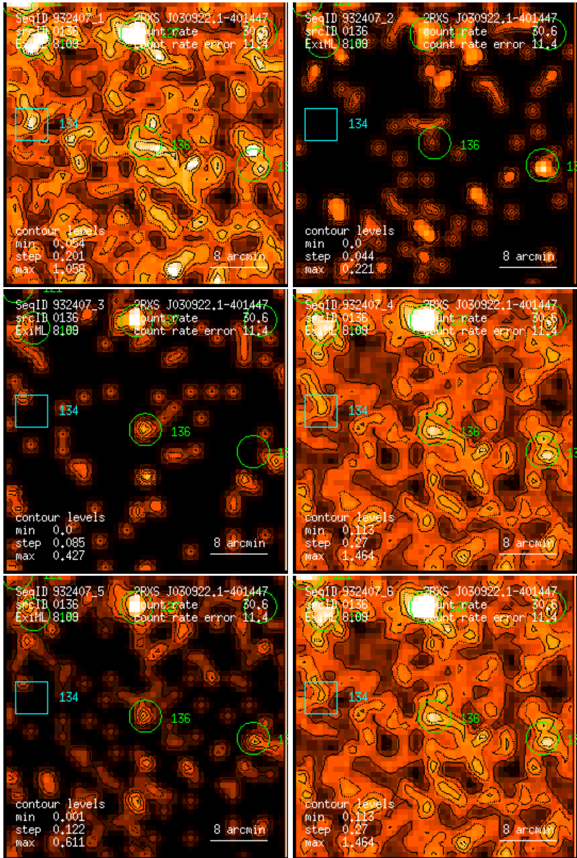
Figure 136: RASS 932407: detection 0136: band rate images, Gaussian filter: (1) PSPC channels 11 – 41, (2) 52 – 90, (3) 91 – 201, (4) 11 – 235, (5) 52 – 201, (6) 11 – 201. Broad band rates in counts/ks. Band rate contour levels in counts/ks/arcmin 2 .
