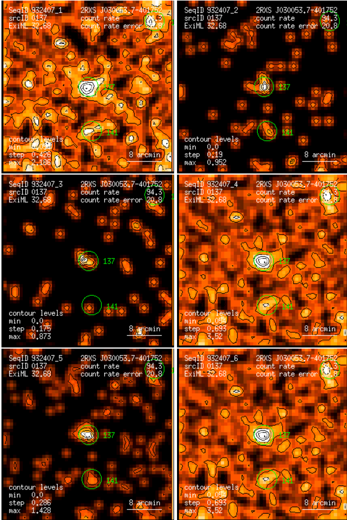
Figure 137: RASS 932407: detection 0137: band rate images, Gaussian filter: (1) PSPC channels 11 – 41, (2) 52 – 90, (3) 91 – 201, (4) 11 – 235, (5) 52 – 201, (6) 11 – 201. Broad band rates in counts/ks. Band rate contour levels in counts/ks/arcmin 2 .
