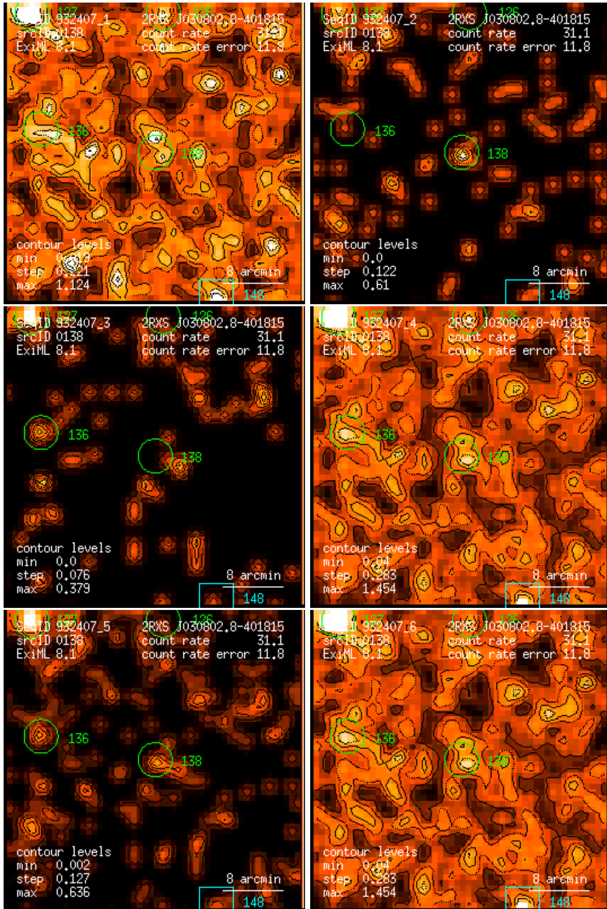
Figure 138: RASS 932407: detection 0138: band rate images, Gaussian filter: (1) PSPC channels 11 – 41, (2) 52 – 90, (3) 91 – 201, (4) 11 – 235, (5) 52 – 201, (6) 11 – 201. Broad band rates in counts/ks. Band rate contour levels in counts/ks/arcmin 2 .
