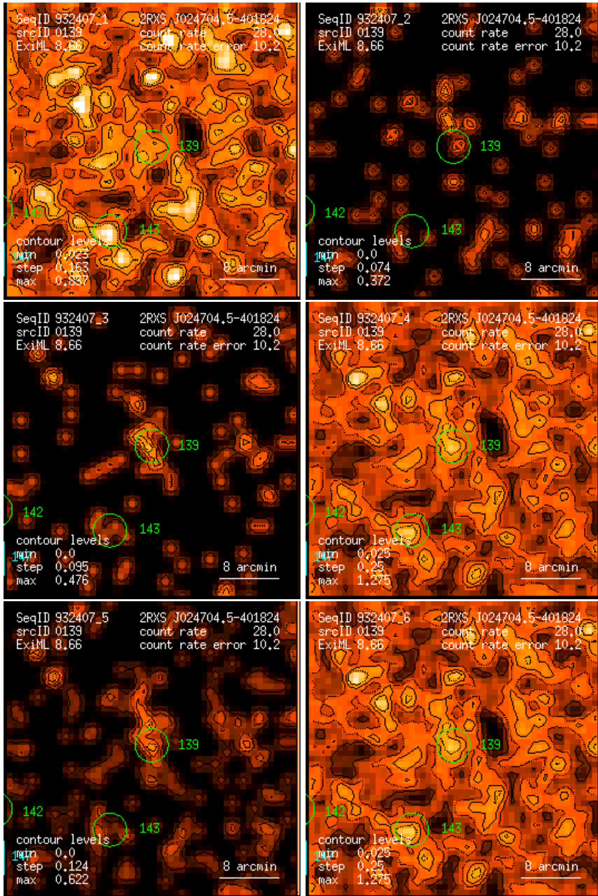
Figure 139: RASS 932407: detection 0139: band rate images, Gaussian filter: (1) PSPC channels 11 – 41, (2) 52 – 90, (3) 91 – 201, (4) 11 – 235, (5) 52 – 201, (6) 11 – 201. Broad band rates in counts/ks. Band rate contour levels in counts/ks/arcmin 2 .
