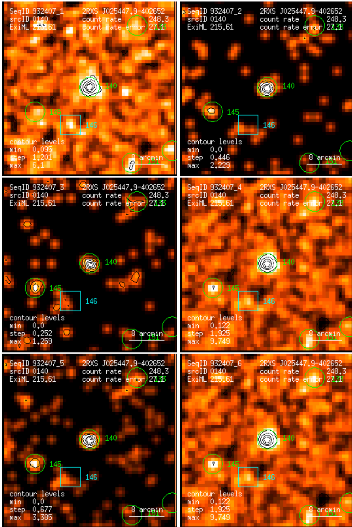
Figure 140: RASS 932407: detection 0140: band rate images, Gaussian filter: (1) PSPC channels 11 – 41, (2) 52 – 90, (3) 91 – 201, (4) 11 – 235, (5) 52 – 201, (6) 11 – 201. Broad band rates in counts/ks. Band rate contour levels in counts/ks/arcmin 2 .
