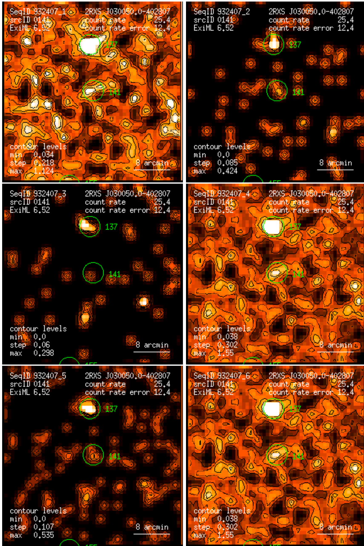
Figure 141: RASS 932407: detection 0141: band rate images, Gaussian filter: (1) PSPC channels 11 – 41, (2) 52 – 90, (3) 91 – 201, (4) 11 – 235, (5) 52 – 201, (6) 11 – 201. Broad band rates in counts/ks. Band rate contour levels in counts/ks/arcmin 2 .
