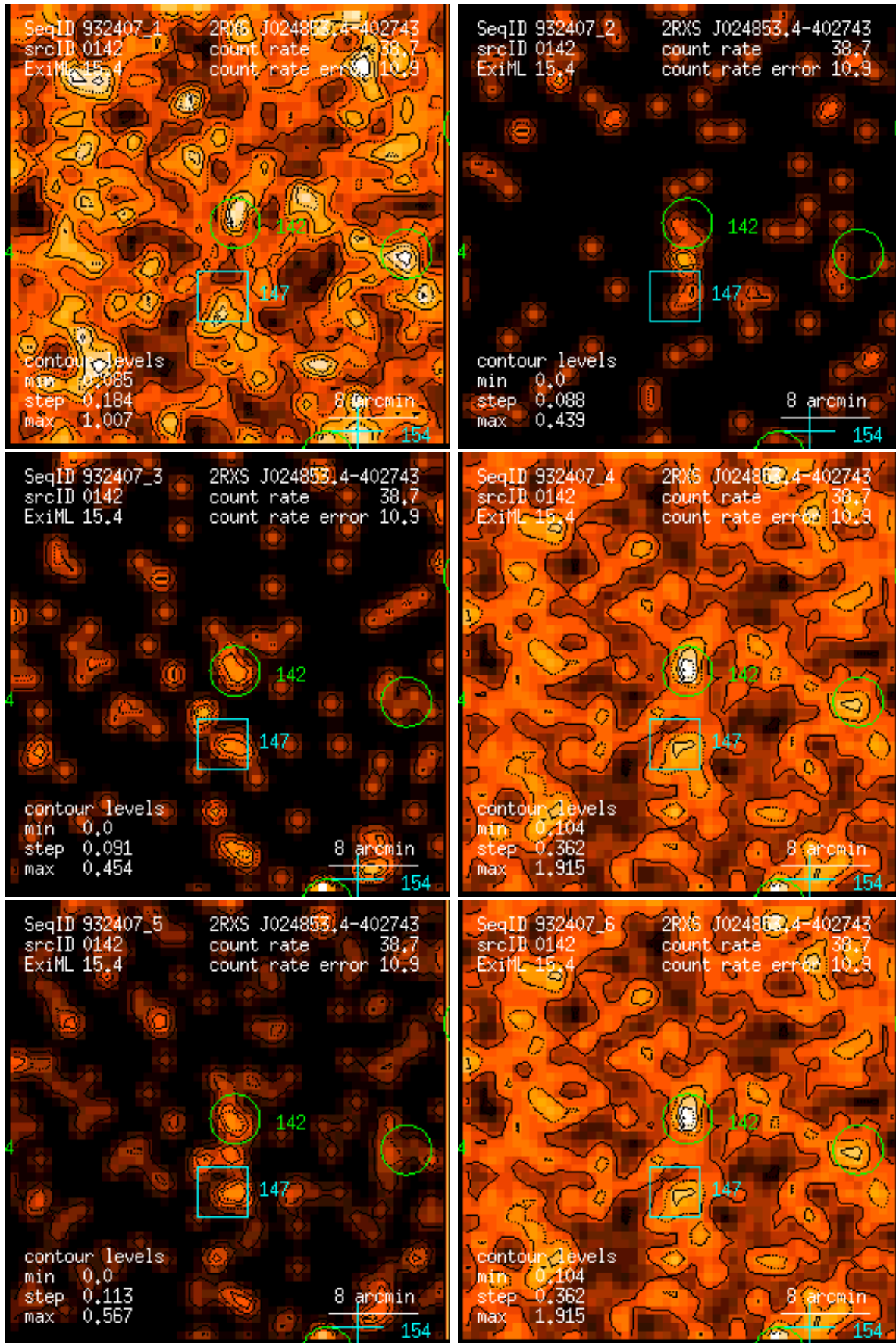
Figure 142: RASS 932407: detection 0142: band rate images, Gaussian filter: (1) PSPC channels 11 – 41, (2) 52 – 90, (3) 91 – 201, (4) 11 – 235, (5) 52 – 201, (6) 11 – 201. Broad band rates in counts/ks. Band rate contour levels in counts/ks/arcmin 2 .
