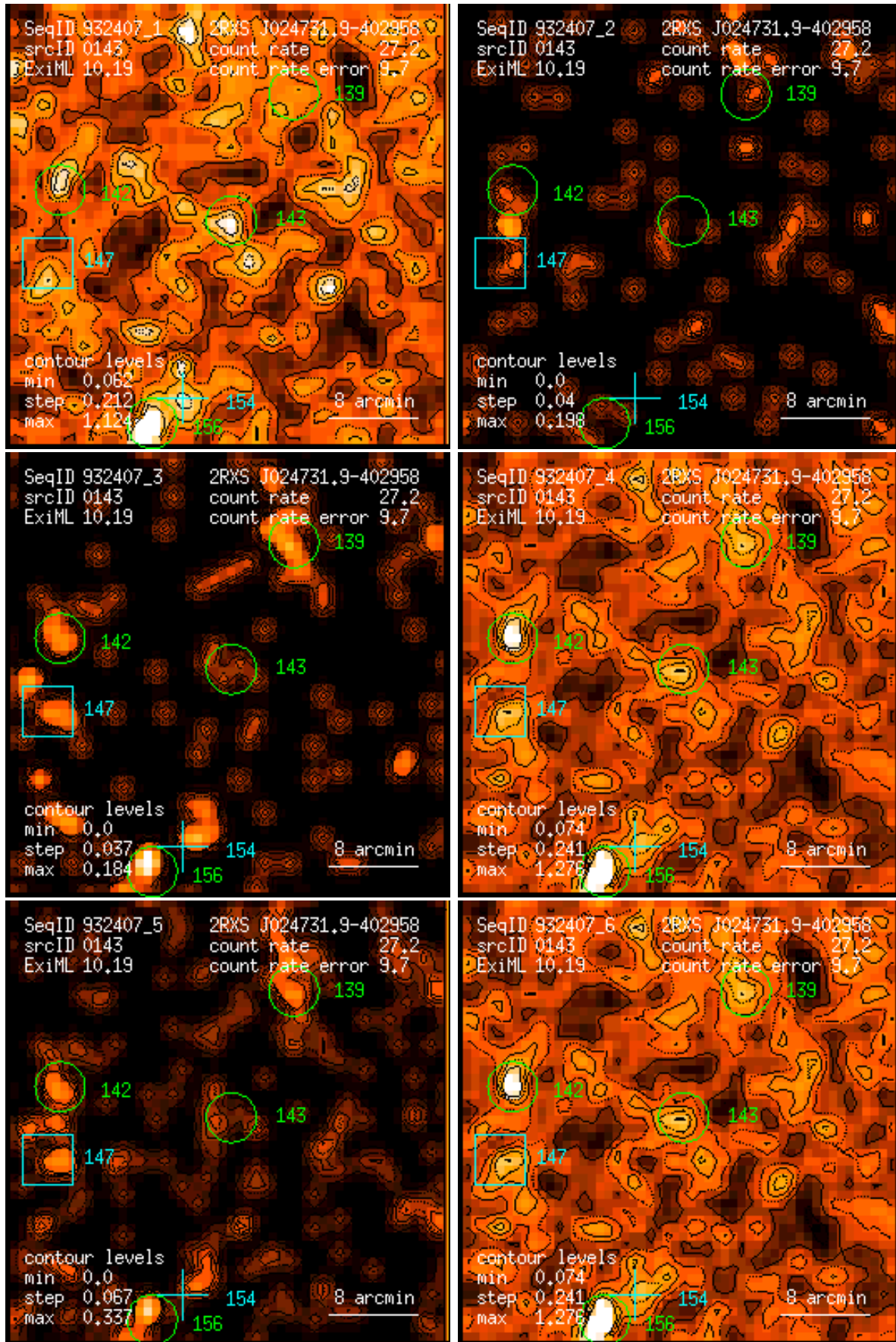
Figure 143: RASS 932407: detection 0143: band rate images, Gaussian filter: (1) PSPC channels 11 – 41, (2) 52 – 90, (3) 91 – 201, (4) 11 – 235, (5) 52 – 201, (6) 11 – 201. Broad band rates in counts/ks. Band rate contour levels in counts/ks/arcmin 2 .
