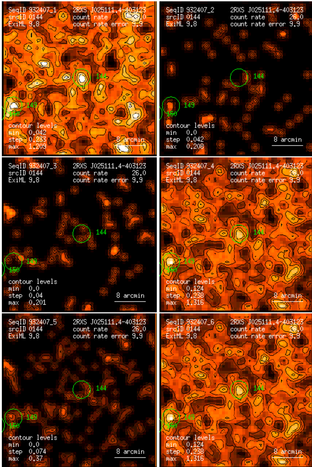
Figure 144: RASS 932407: detection 0144: band rate images, Gaussian filter: (1) PSPC channels 11 – 41, (2) 52 – 90, (3) 91 – 201, (4) 11 – 235, (5) 52 – 201, (6) 11 – 201. Broad band rates in counts/ks. Band rate contour levels in counts/ks/arcmin 2 .
