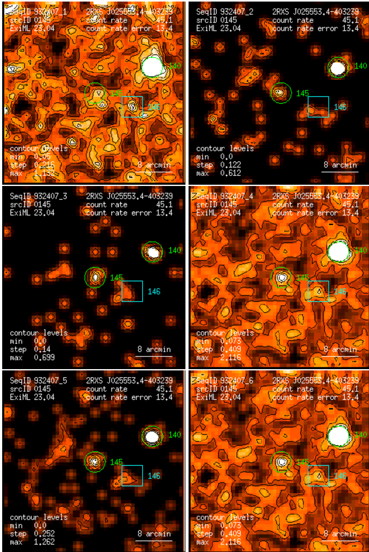
Figure 145: RASS 932407: detection 0145: band rate images, Gaussian filter: (1) PSPC channels 11 – 41, (2) 52 – 90, (3) 91 – 201, (4) 11 – 235, (5) 52 – 201, (6) 11 – 201. Broad band rates in counts/ks. Band rate contour levels in counts/ks/arcmin 2 .
