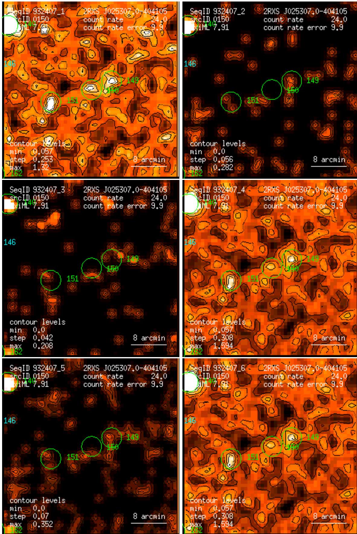
Figure 150: RASS 932407: detection 0150: band rate images, Gaussian filter: (1) PSPC channels 11 – 41, (2) 52 – 90, (3) 91 – 201, (4) 11 – 235, (5) 52 – 201, (6) 11 – 201. Broad band rates in counts/ks. Band rate contour levels in counts/ks/arcmin 2 .
