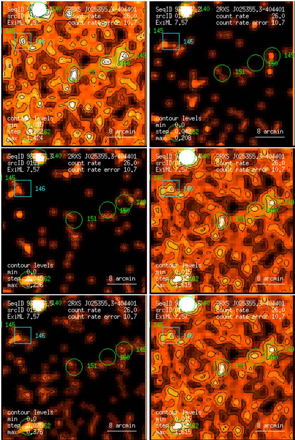
Figure 151: RASS 932407: detection 0151: band rate images, Gaussian filter: (1) PSPC channels 11 – 41, (2) 52 – 90, (3) 91 – 201, (4) 11 – 235, (5) 52 – 201, (6) 11 – 201. Broad band rates in counts/ks. Band rate contour levels in counts/ks/arcmin 2 .
