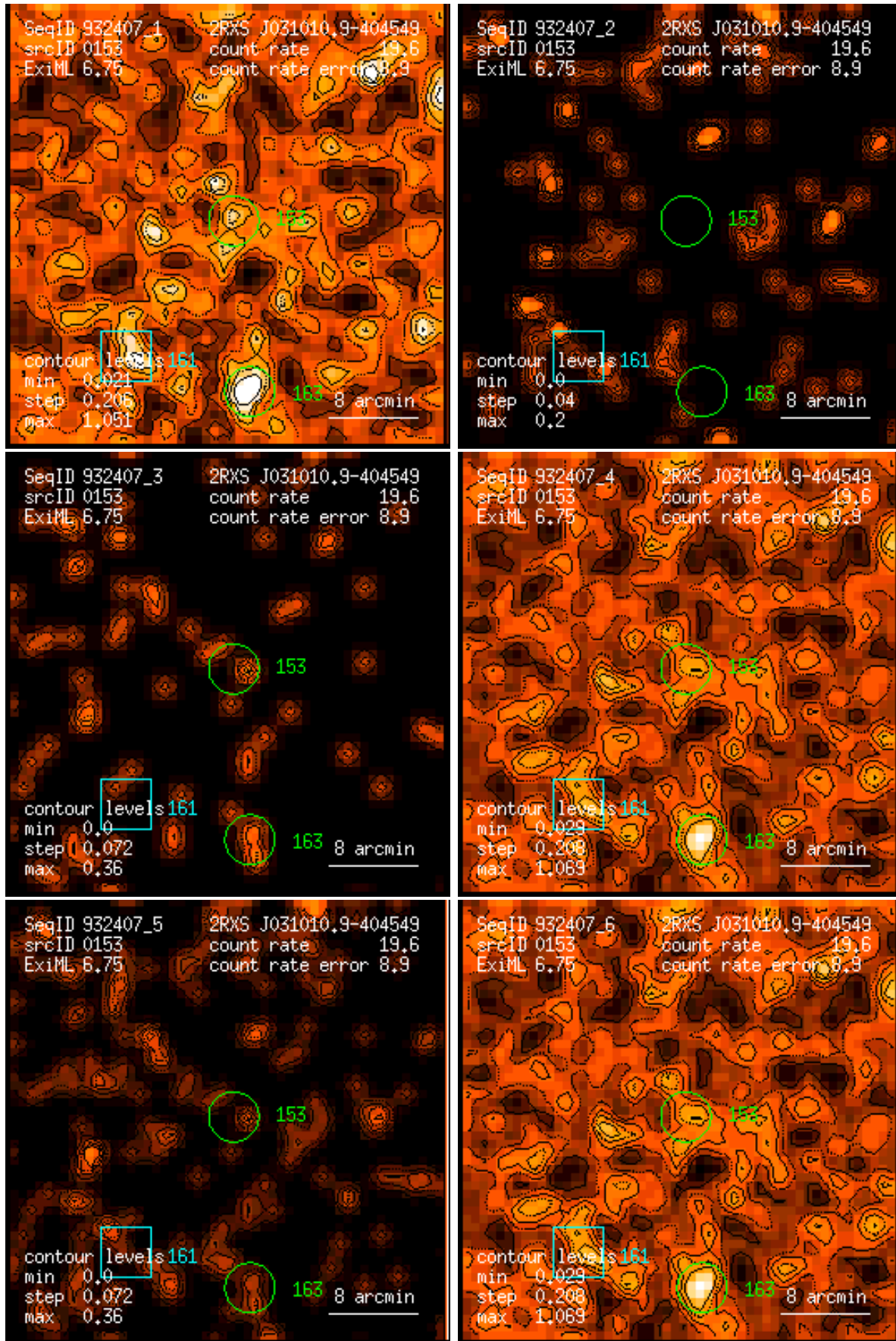
Figure 153: RASS 932407: detection 0153: band rate images, Gaussian filter: (1) PSPC channels 11 – 41, (2) 52 – 90, (3) 91 – 201, (4) 11 – 235, (5) 52 – 201, (6) 11 – 201. Broad band rates in counts/ks. Band rate contour levels in counts/ks/arcmin 2 .
