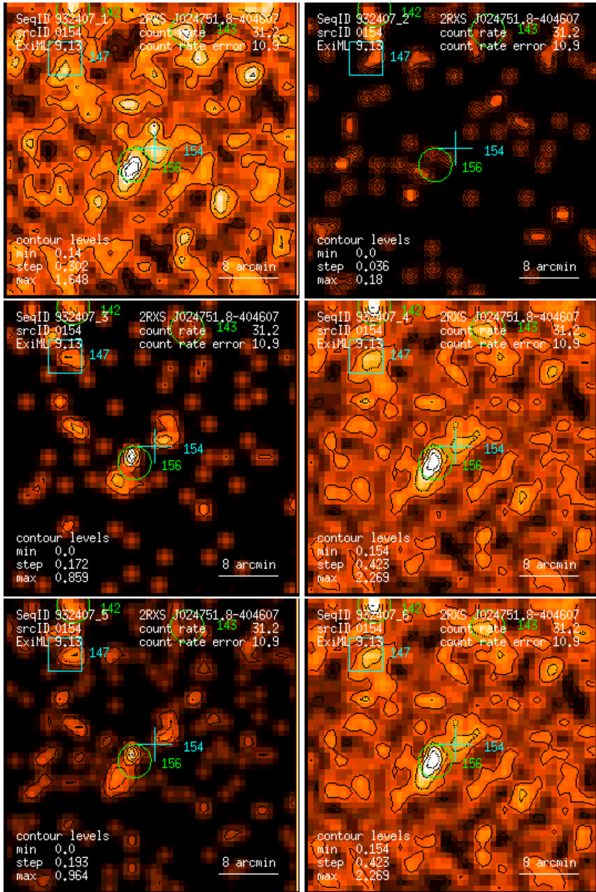
Figure 154: RASS 932407: detection 0154: band rate images, Gaussian filter: (1) PSPC channels 11 – 41, (2) 52 – 90, (3) 91 – 201, (4) 11 – 235, (5) 52 – 201, (6) 11 – 201. Broad band rates in counts/ks. Band rate contour levels in counts/ks/arcmin 2 .
