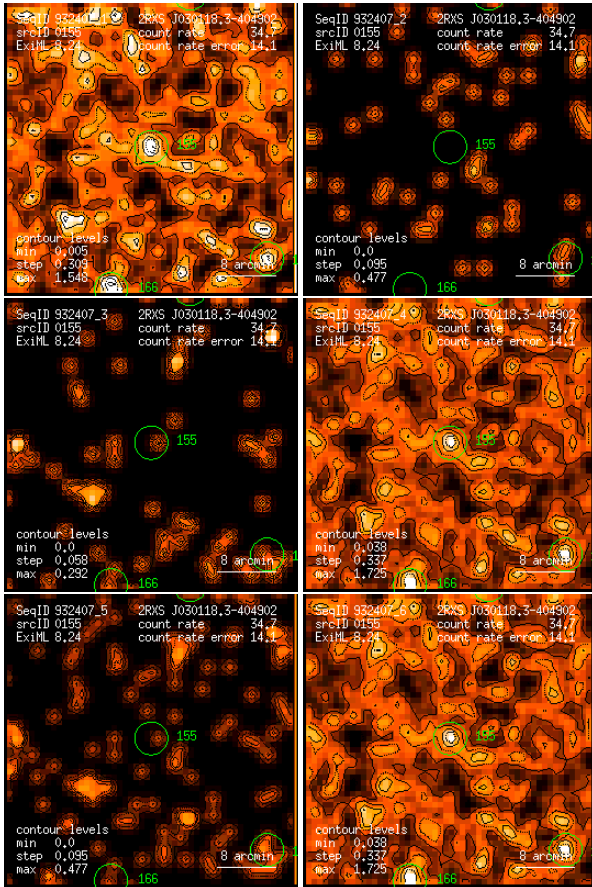
Figure 155: RASS 932407: detection 0155: band rate images, Gaussian filter: (1) PSPC channels 11 – 41, (2) 52 – 90, (3) 91 – 201, (4) 11 – 235, (5) 52 – 201, (6) 11 – 201. Broad band rates in counts/ks. Band rate contour levels in counts/ks/arcmin 2 .
