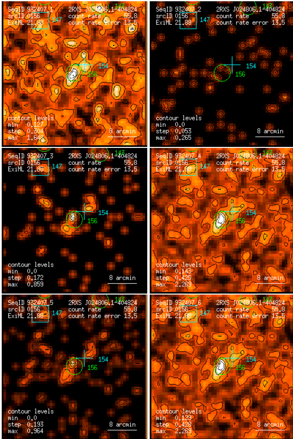
Figure 156: RASS 932407: detection 0156: band rate images, Gaussian filter: (1) PSPC channels 11 – 41, (2) 52 – 90, (3) 91 – 201, (4) 11 – 235, (5) 52 – 201, (6) 11 – 201. Broad band rates in counts/ks. Band rate contour levels in counts/ks/arcmin 2 .
