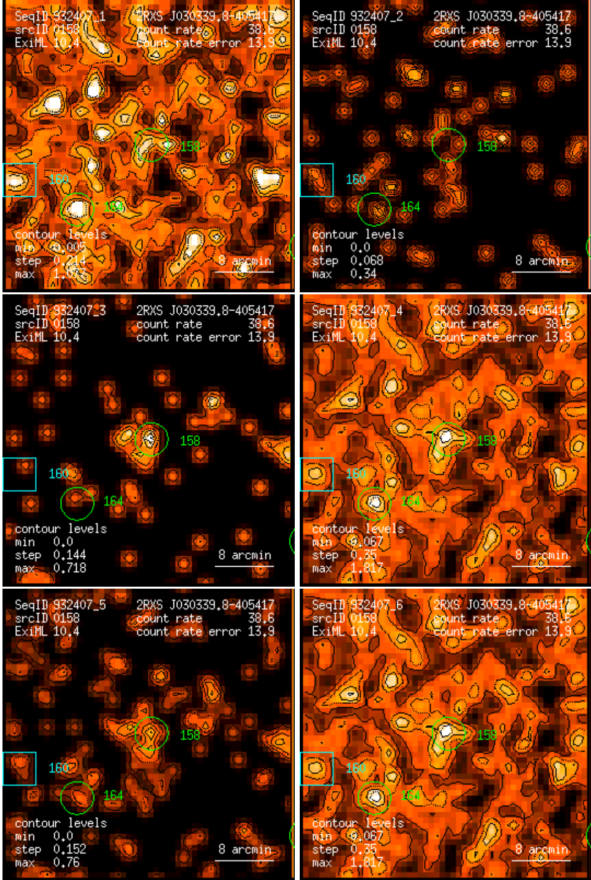
Figure 158: RASS 932407: detection 0158: band rate images, Gaussian filter: (1) PSPC channels 11 – 41, (2) 52 – 90, (3) 91 – 201, (4) 11 – 235, (5) 52 – 201, (6) 11 – 201. Broad band rates in counts/ks. Band rate contour levels in counts/ks/arcmin 2 .
