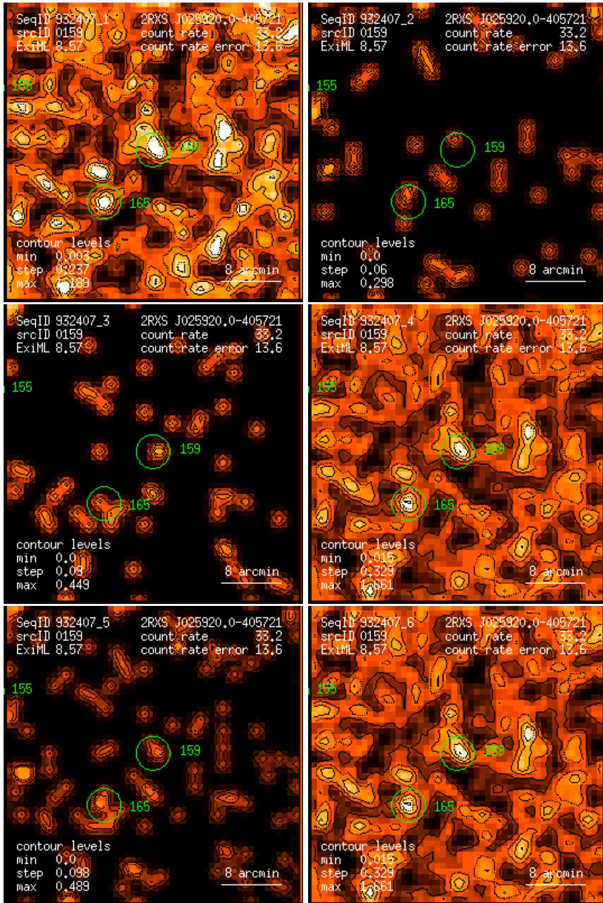
Figure 159: RASS 932407: detection 0159: band rate images, Gaussian filter: (1) PSPC channels 11 – 41, (2) 52 – 90, (3) 91 – 201, (4) 11 – 235, (5) 52 – 201, (6) 11 – 201. Broad band rates in counts/ks. Band rate contour levels in counts/ks/arcmin 2 .
