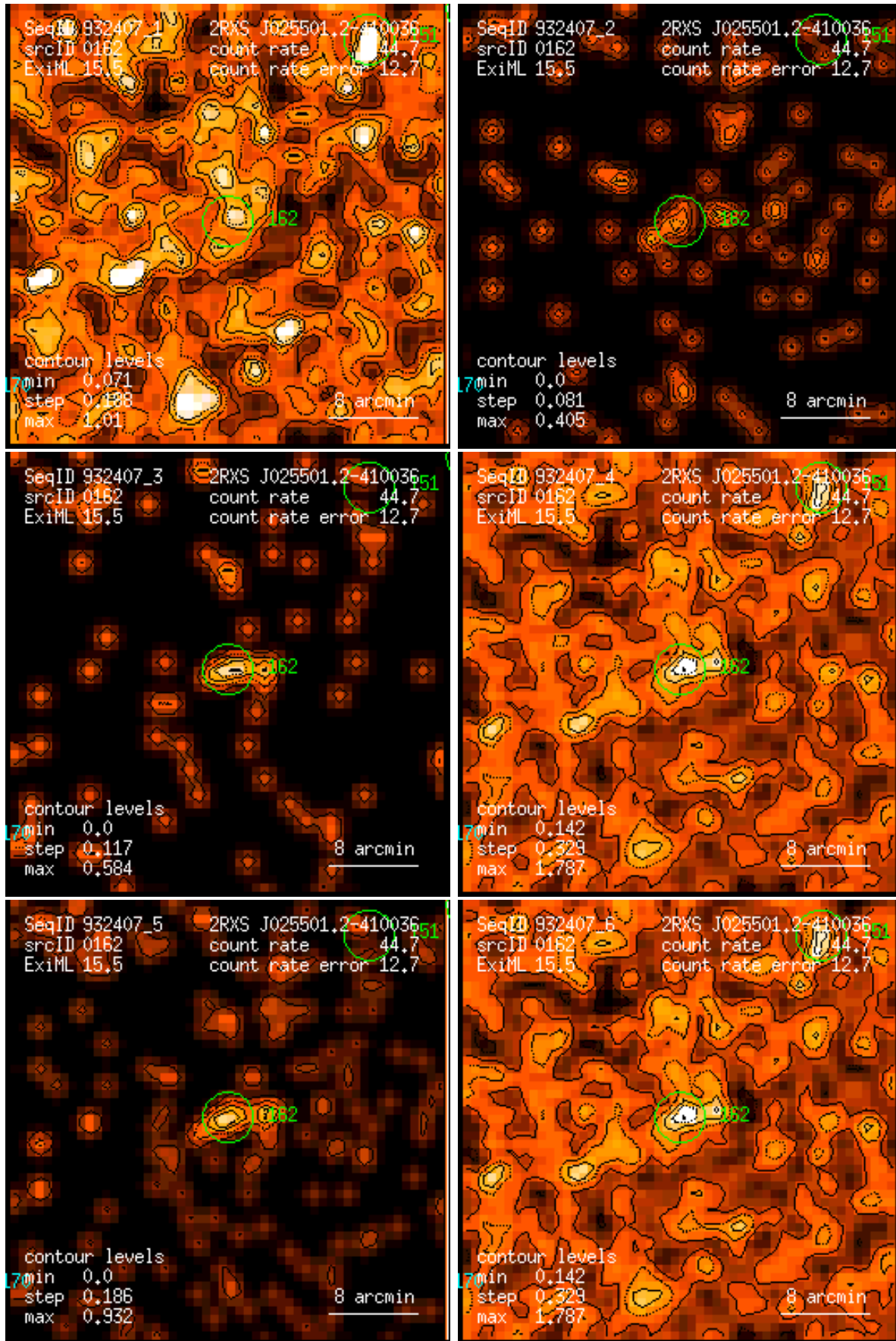
Figure 162: RASS 932407: detection 0162: band rate images, Gaussian filter: (1) PSPC channels 11 – 41, (2) 52 – 90, (3) 91 – 201, (4) 11 – 235, (5) 52 – 201, (6) 11 – 201. Broad band rates in counts/ks. Band rate contour levels in counts/ks/arcmin 2 .
