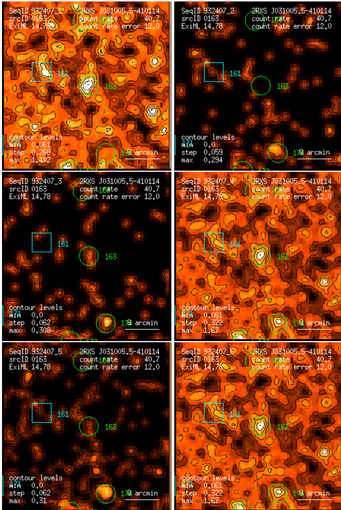
Figure 163: RASS 932407: detection 0163: band rate images, Gaussian filter: (1) PSPC channels 11 – 41, (2) 52 – 90, (3) 91 – 201, (4) 11 – 235, (5) 52 – 201, (6) 11 – 201. Broad band rates in counts/ks. Band rate contour levels in counts/ks/arcmin 2 .
