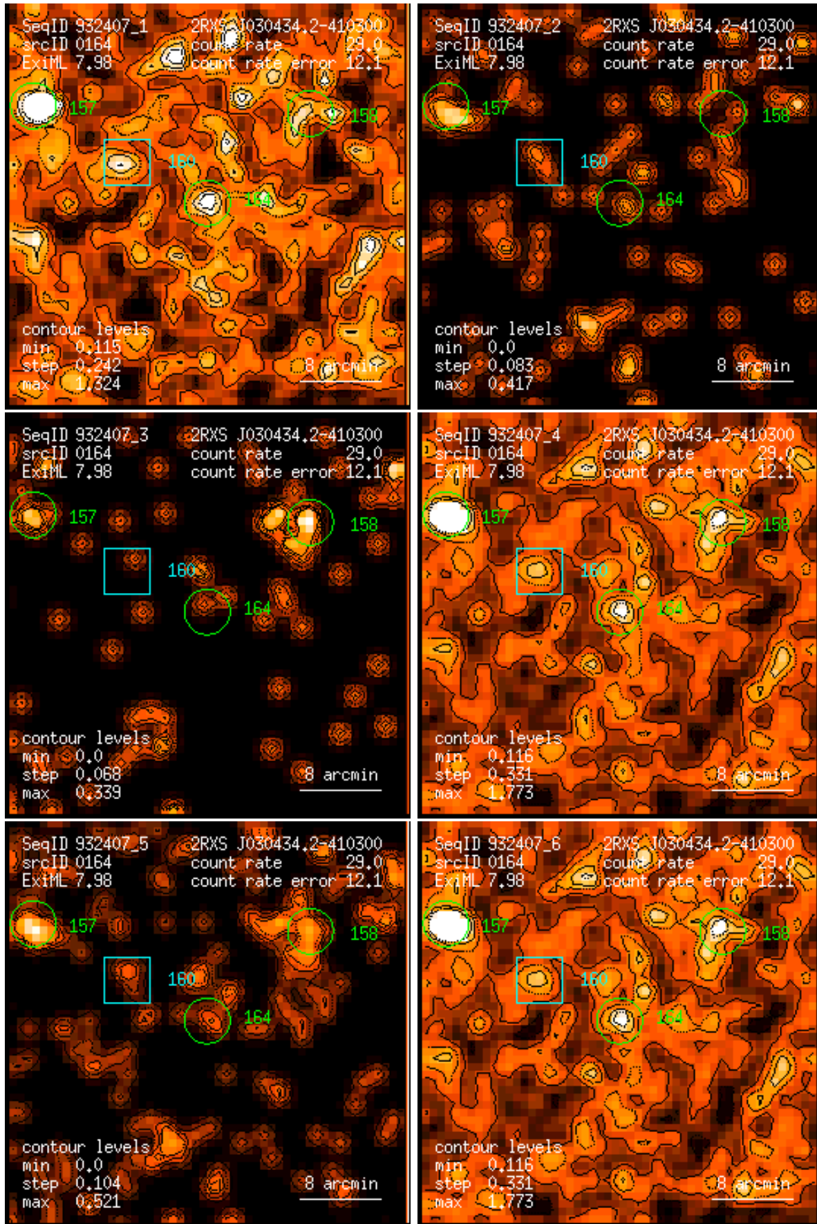
Figure 164: RASS 932407: detection 0164: band rate images, Gaussian filter: (1) PSPC channels 11 – 41, (2) 52 – 90, (3) 91 – 201, (4) 11 – 235, (5) 52 – 201, (6) 11 – 201. Broad band rates in counts/ks. Band rate contour levels in counts/ks/arcmin 2 .
