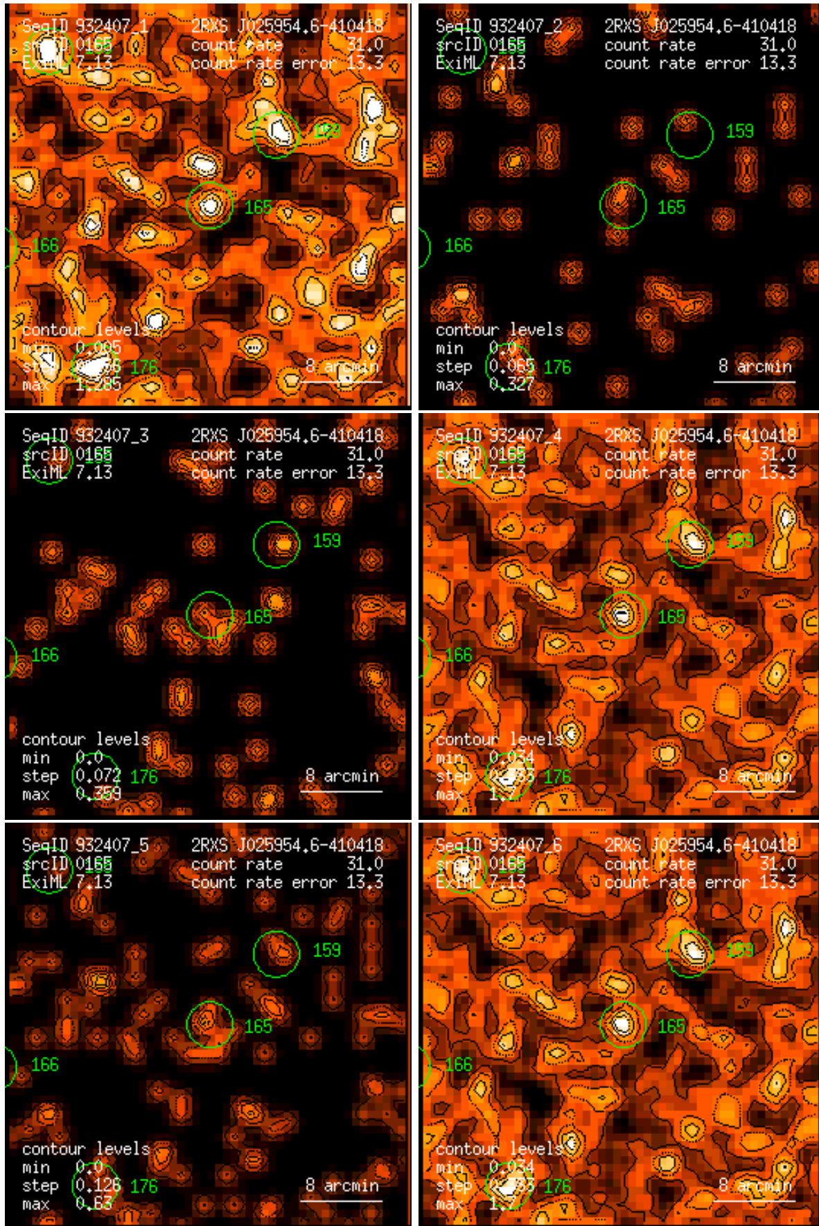
Figure 165: RASS 932407: detection 0165: band rate images, Gaussian filter: (1) PSPC channels 11 – 41, (2) 52 – 90, (3) 91 – 201, (4) 11 – 235, (5) 52 – 201, (6) 11 – 201. Broad band rates in counts/ks. Band rate contour levels in counts/ks/arcmin 2 .
