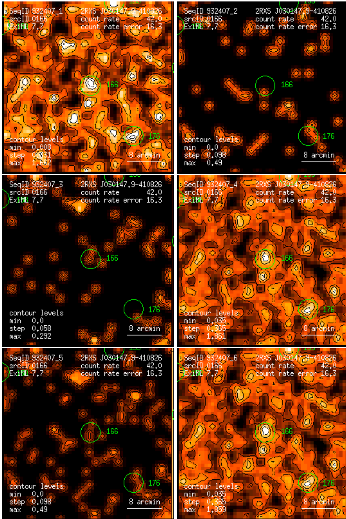
Figure 166: RASS 932407: detection 0166: band rate images, Gaussian filter: (1) PSPC channels 11 – 41, (2) 52 – 90, (3) 91 – 201, (4) 11 – 235, (5) 52 – 201, (6) 11 – 201. Broad band rates in counts/ks. Band rate contour levels in counts/ks/arcmin 2 .
