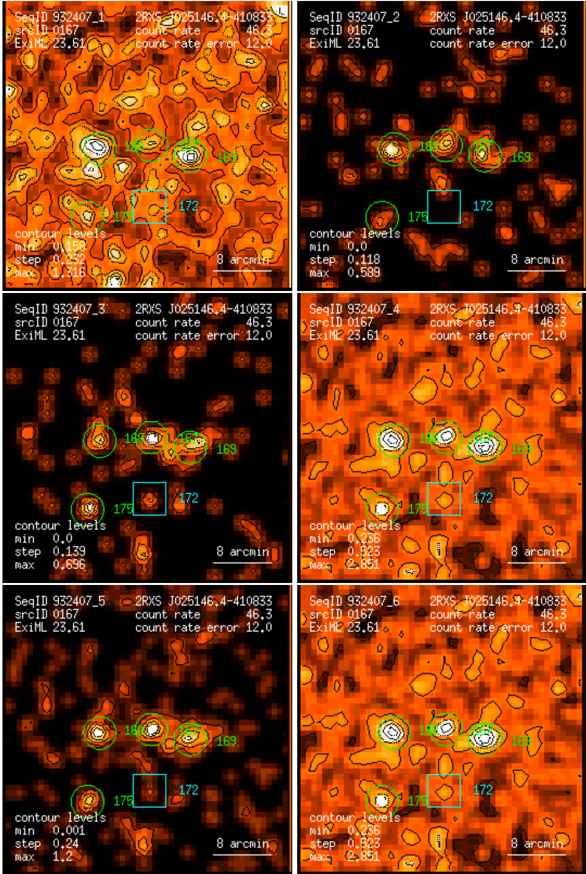
Figure 167: RASS 932407: detection 0167: band rate images, Gaussian filter: (1) PSPC channels 11 – 41, (2) 52 – 90, (3) 91 – 201, (4) 11 – 235, (5) 52 – 201, (6) 11 – 201. Broad band rates in counts/ks. Band rate contour levels in counts/ks/arcmin 2 .
