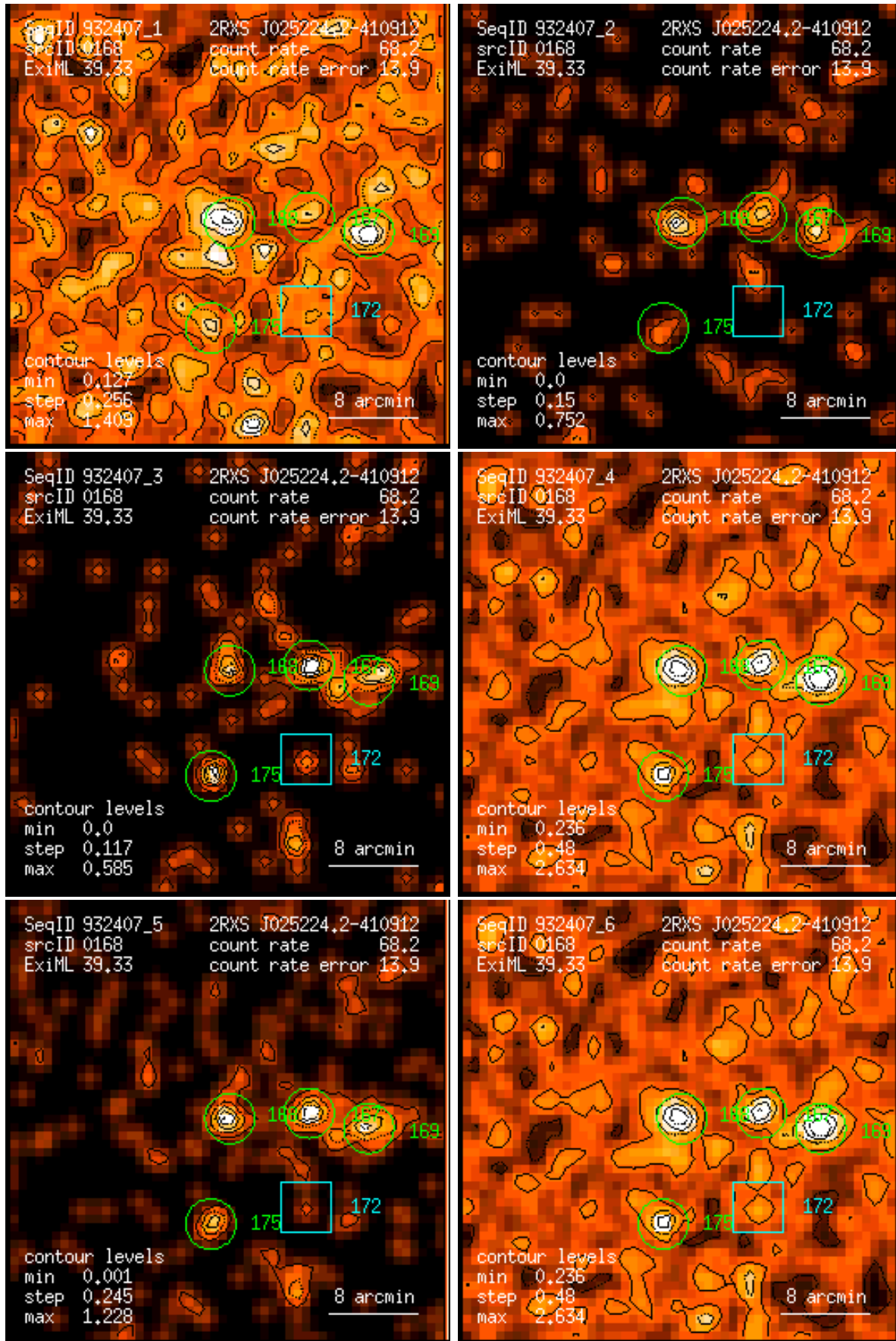
Figure 168: RASS 932407: detection 0168: band rate images, Gaussian filter: (1) PSPC channels 11 – 41, (2) 52 – 90, (3) 91 – 201, (4) 11 – 235, (5) 52 – 201, (6) 11 – 201. Broad band rates in counts/ks. Band rate contour levels in counts/ks/arcmin 2 .
