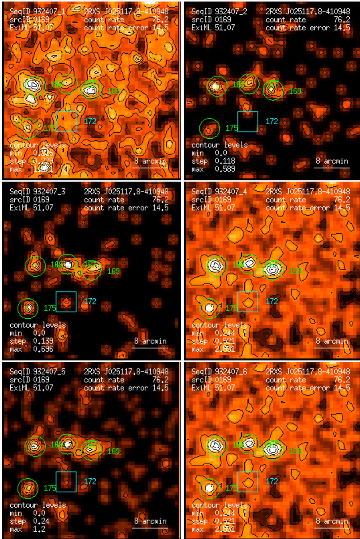
Figure 169: RASS 932407: detection 0169: band rate images, Gaussian filter: (1) PSPC channels 11 – 41, (2) 52 – 90, (3) 91 – 201, (4) 11 – 235, (5) 52 – 201, (6) 11 – 201. Broad band rates in counts/ks. Band rate contour levels in counts/ks/arcmin 2 .
