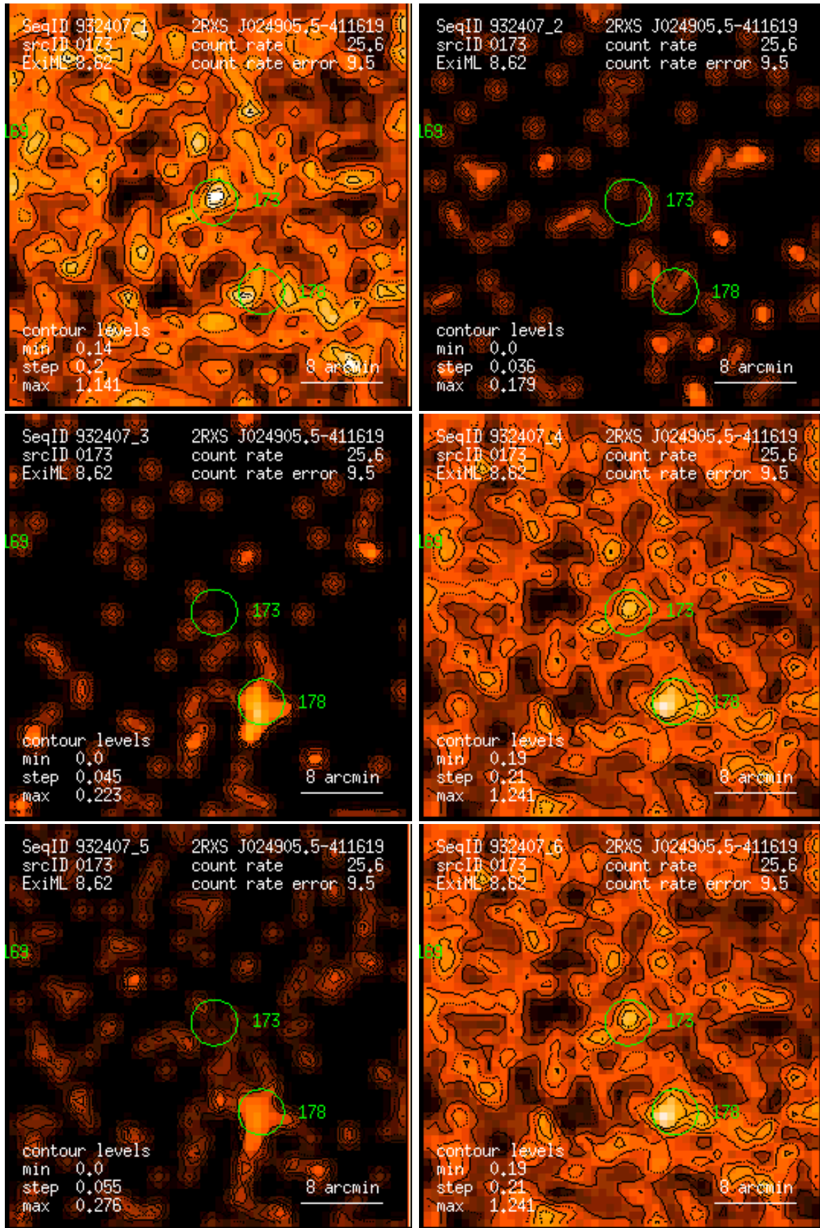
Figure 173: RASS 932407: detection 0173: band rate images, Gaussian filter: (1) PSPC channels 11 – 41, (2) 52 – 90, (3) 91 – 201, (4) 11 – 235, (5) 52 – 201, (6) 11 – 201. Broad band rates in counts/ks. Band rate contour levels in counts/ks/arcmin 2 .
