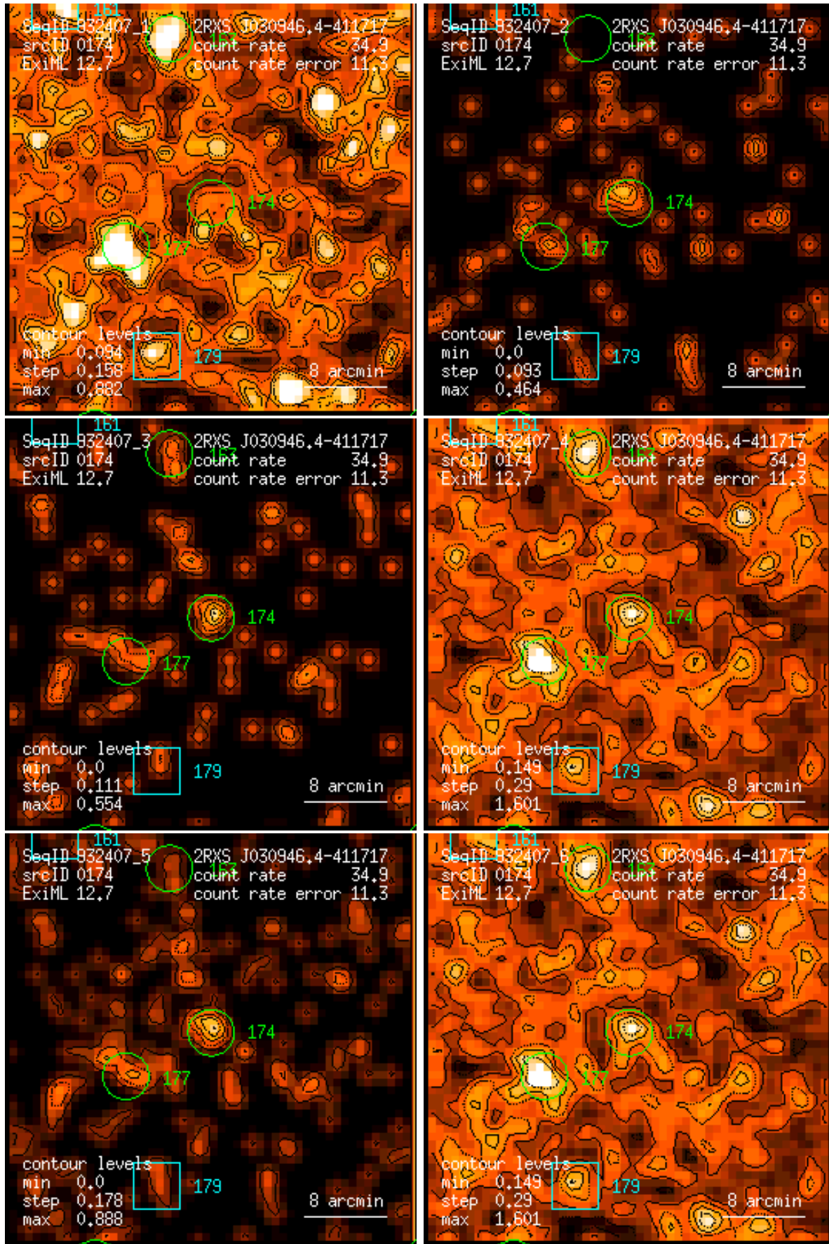
Figure 174: RASS 932407: detection 0174: band rate images, Gaussian filter: (1) PSPC channels 11 – 41, (2) 52 – 90, (3) 91 – 201, (4) 11 – 235, (5) 52 – 201, (6) 11 – 201. Broad band rates in counts/ks. Band rate contour levels in counts/ks/arcmin 2 .
