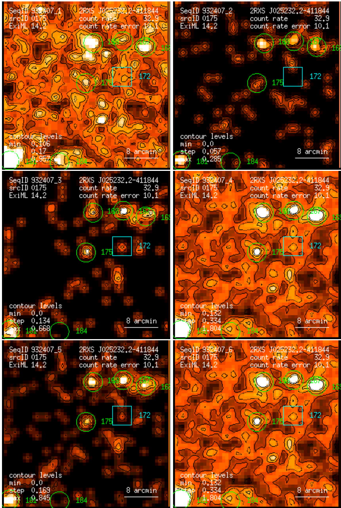
Figure 175: RASS 932407: detection 0175: band rate images, Gaussian filter: (1) PSPC channels 11 – 41, (2) 52 – 90, (3) 91 – 201, (4) 11 – 235, (5) 52 – 201, (6) 11 – 201. Broad band rates in counts/ks. Band rate contour levels in counts/ks/arcmin 2 .
