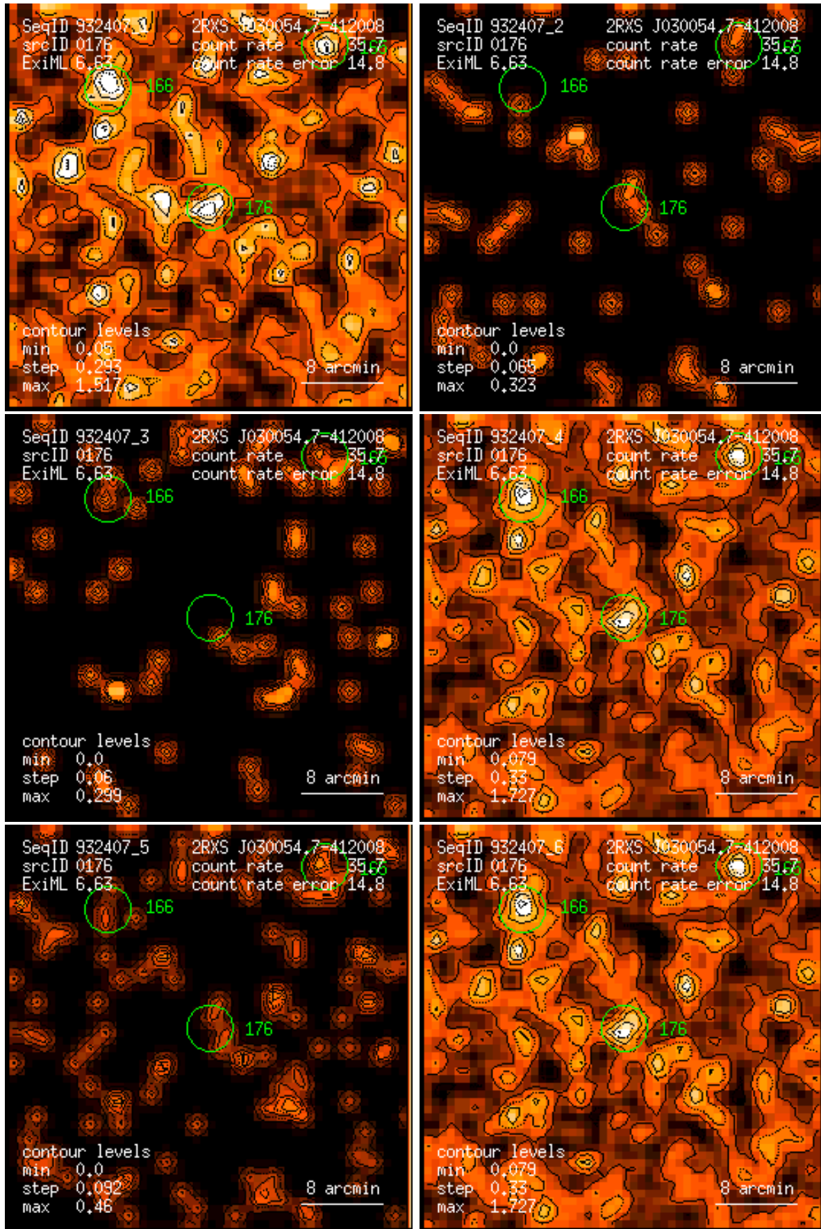
Figure 176: RASS 932407: detection 0176: band rate images, Gaussian filter: (1) PSPC channels 11 – 41, (2) 52 – 90, (3) 91 – 201, (4) 11 – 235, (5) 52 – 201, (6) 11 – 201. Broad band rates in counts/ks. Band rate contour levels in counts/ks/arcmin 2 .
