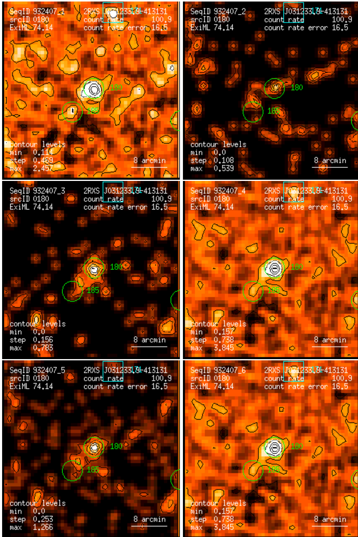
Figure 180: RASS 932407: detection 0180: band rate images, Gaussian filter: (1) PSPC channels 11 – 41, (2) 52 – 90, (3) 91 – 201, (4) 11 – 235, (5) 52 – 201, (6) 11 – 201. Broad band rates in counts/ks. Band rate contour levels in counts/ks/arcmin 2 .
