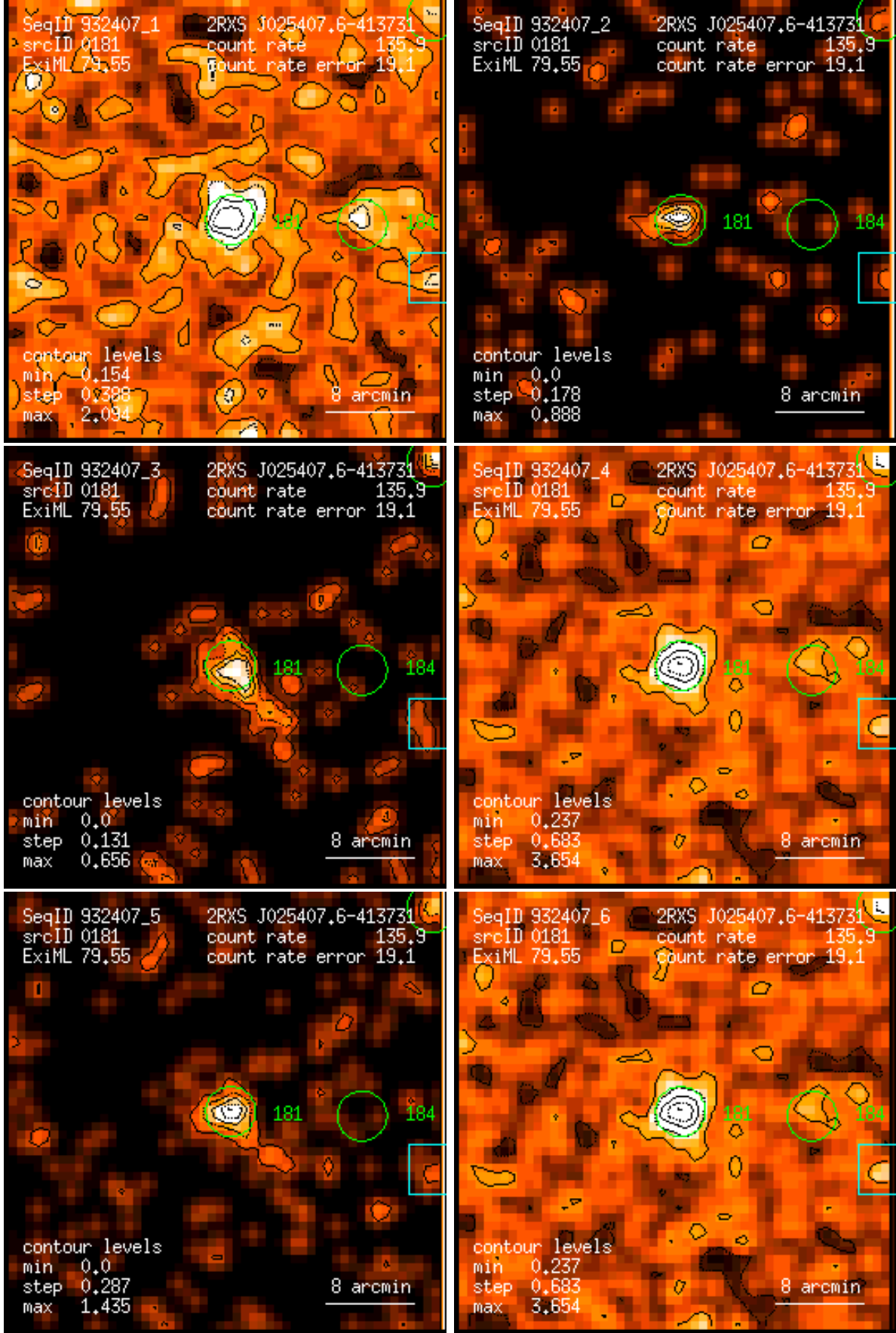
Figure 181: RASS 932407: detection 0181: band rate images, Gaussian filter: (1) PSPC channels 11 – 41, (2) 52 – 90, (3) 91 – 201, (4) 11 – 235, (5) 52 – 201, (6) 11 – 201. Broad band rates in counts/ks. Band rate contour levels in counts/ks/arcmin 2 .
