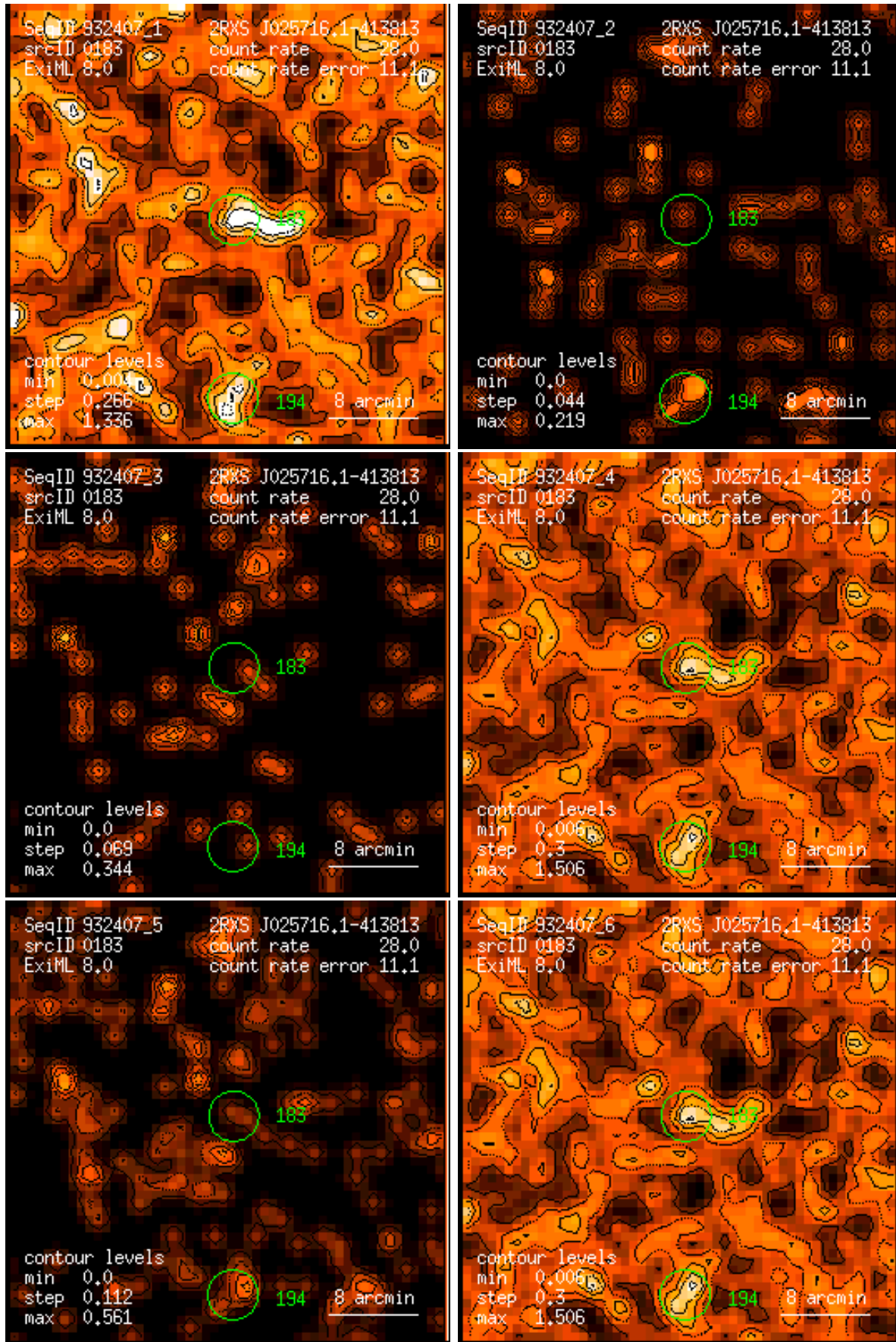
Figure 183: RASS 932407: detection 0183: band rate images, Gaussian filter: (1) PSPC channels 11 – 41, (2) 52 – 90, (3) 91 – 201, (4) 11 – 235, (5) 52 – 201, (6) 11 – 201. Broad band rates in counts/ks. Band rate contour levels in counts/ks/arcmin 2 .
